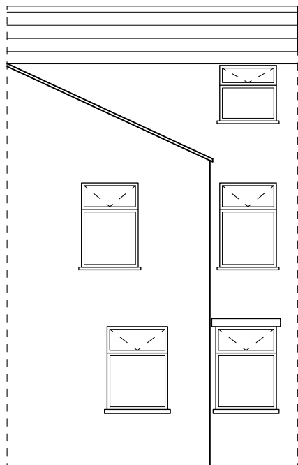
SOUTH WEST ELEVATION SCALE 1:100 PROPOSED - P008
