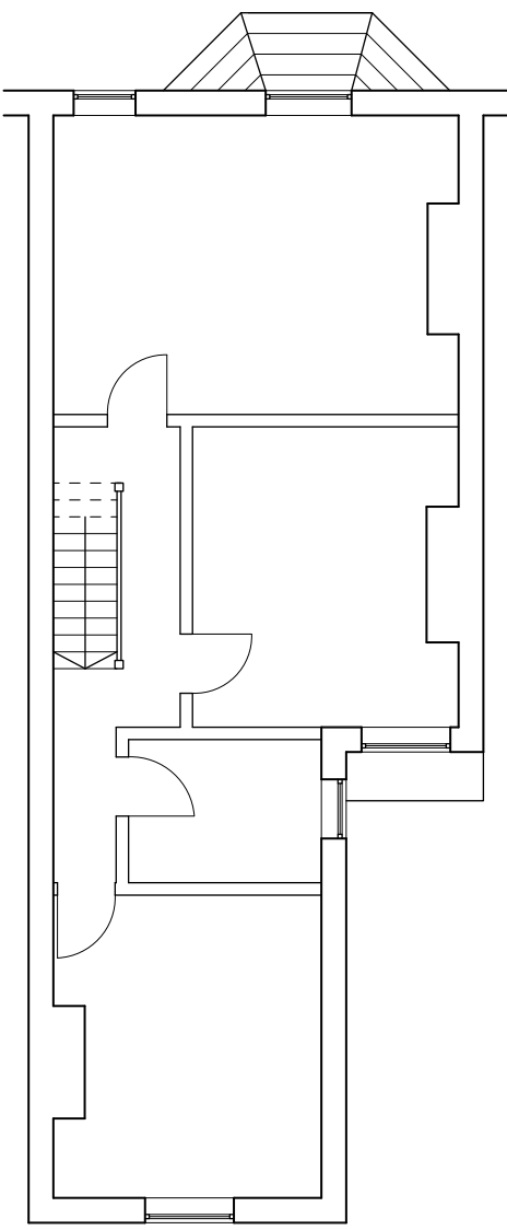
FIRST FLOOR SCALE 1:100 EXISTING - E004
