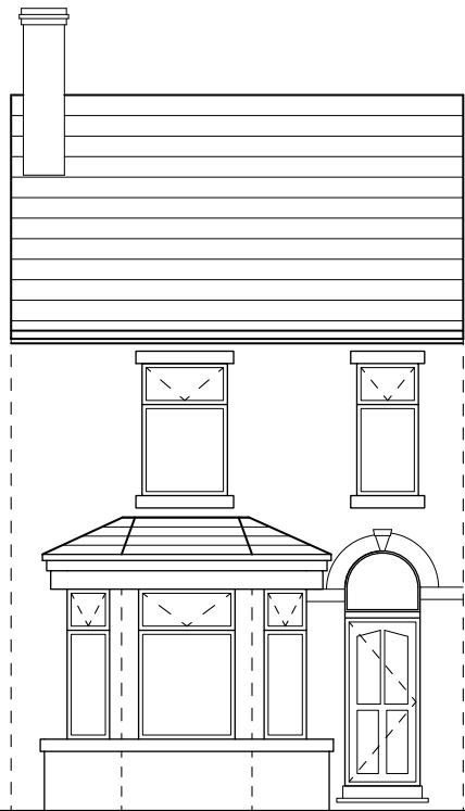
NORTH EAST ELEVATION SCALE 1:100 EXISTING - E006
