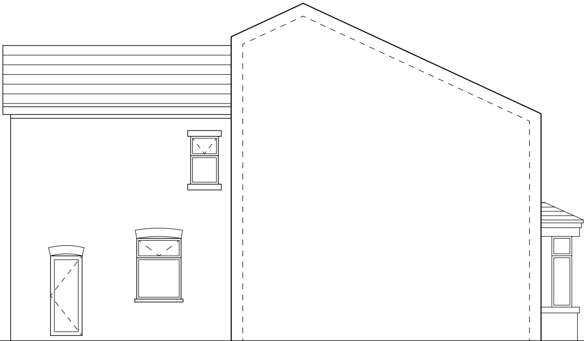
SOUTH EAST ELEVATION SCALE 1:100 EXISTING - E007
