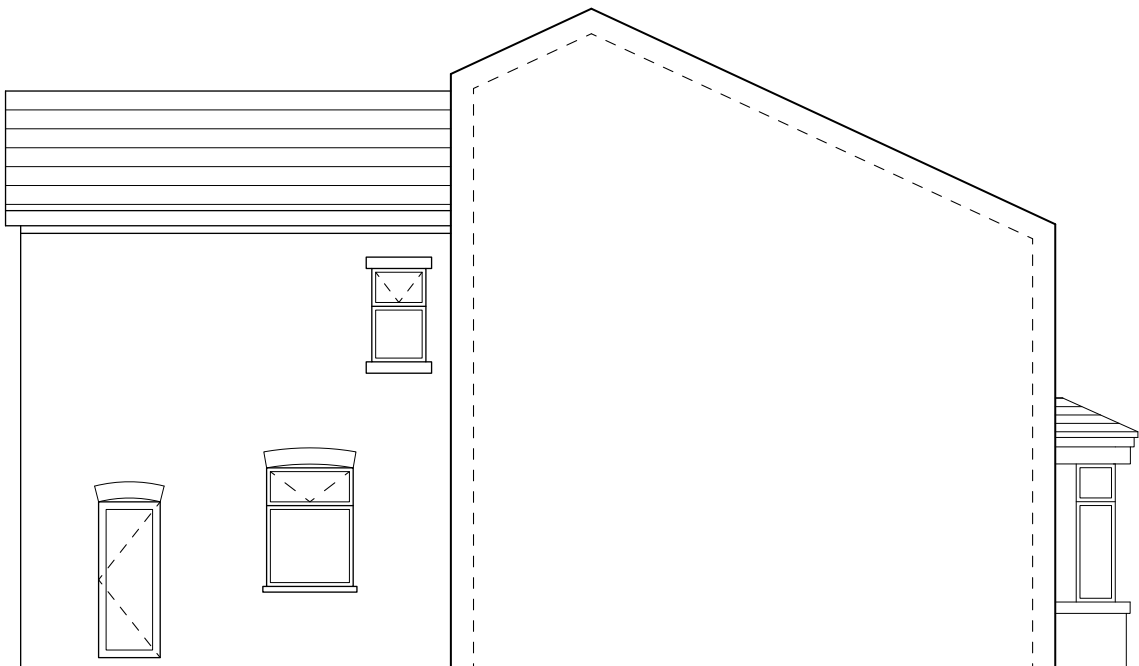
SOUTH EAST ELEVATION SCALE 1:100 PROPOSED - P007
