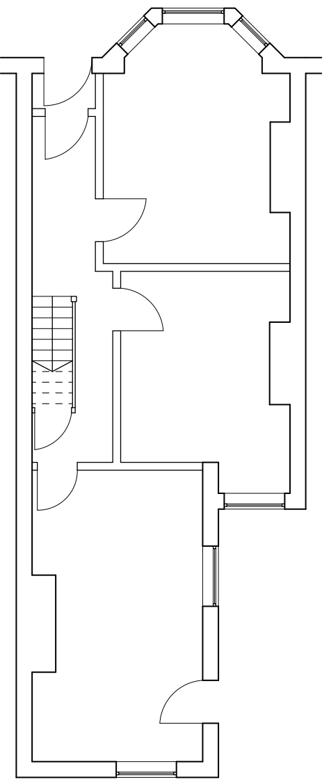
GROUND FLOOR SCALE 1:100 EXISTING - E003
