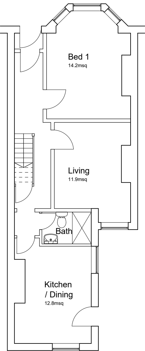
GROUND FLOOR SCALE 1:100 PROPOSED - P003
