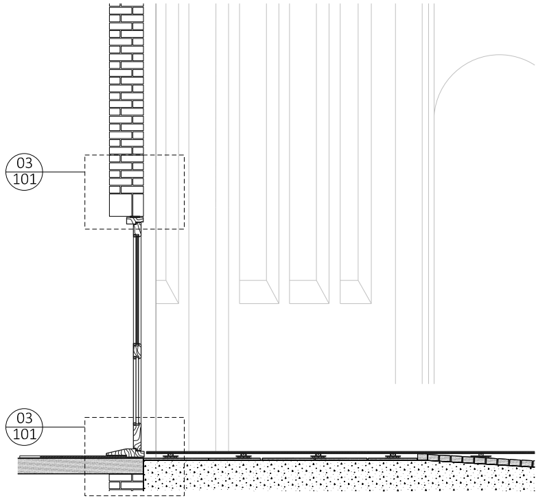
01 Proposed Timber Framed Glass Door Section
