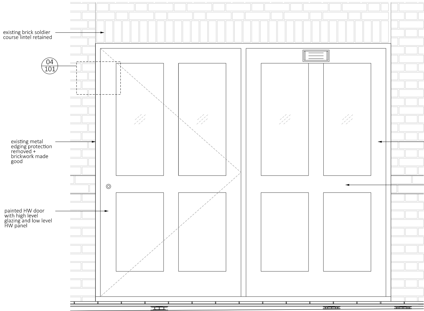
02 Proposed Timber Framed Glass Door Elevation
