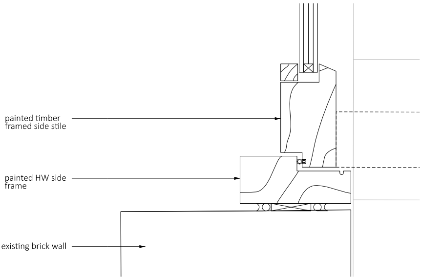
04 Proposed External Timber Glazing Side Detail - 1:5
