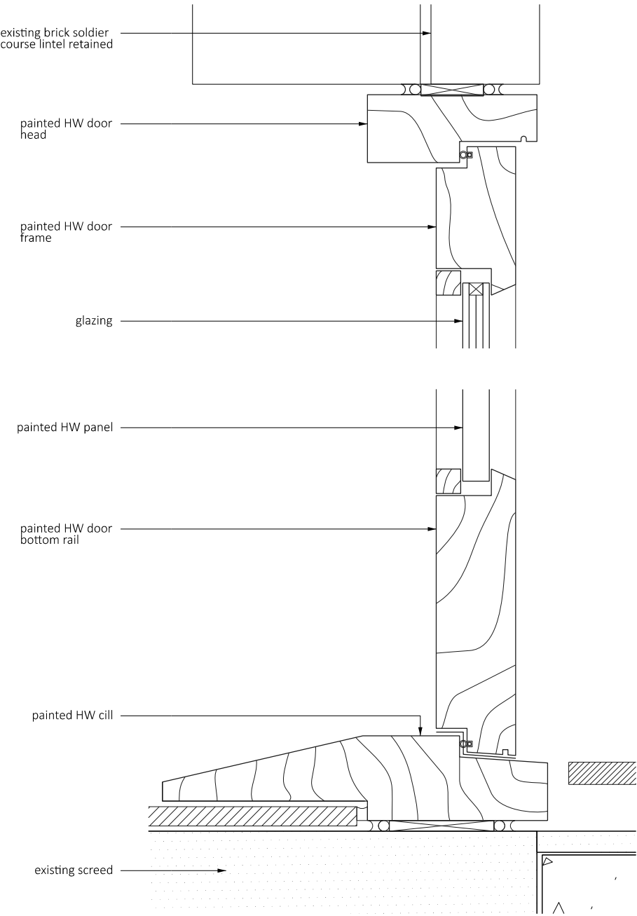
03 Proposed Timber Framed Glass Door Head and Cill Detail - 1:5
