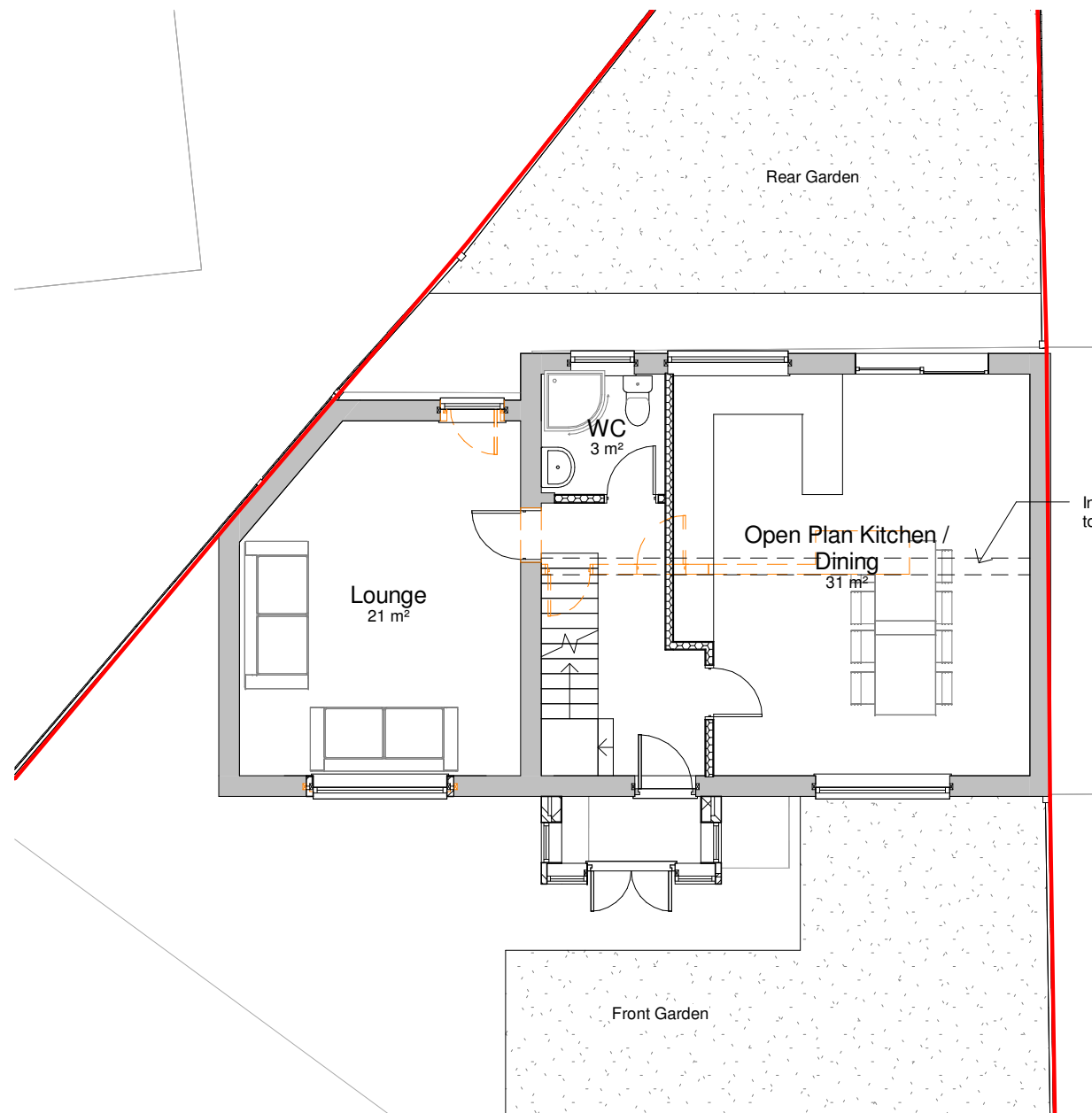
1 Proposed Ground Floor Plan 1 : 100
