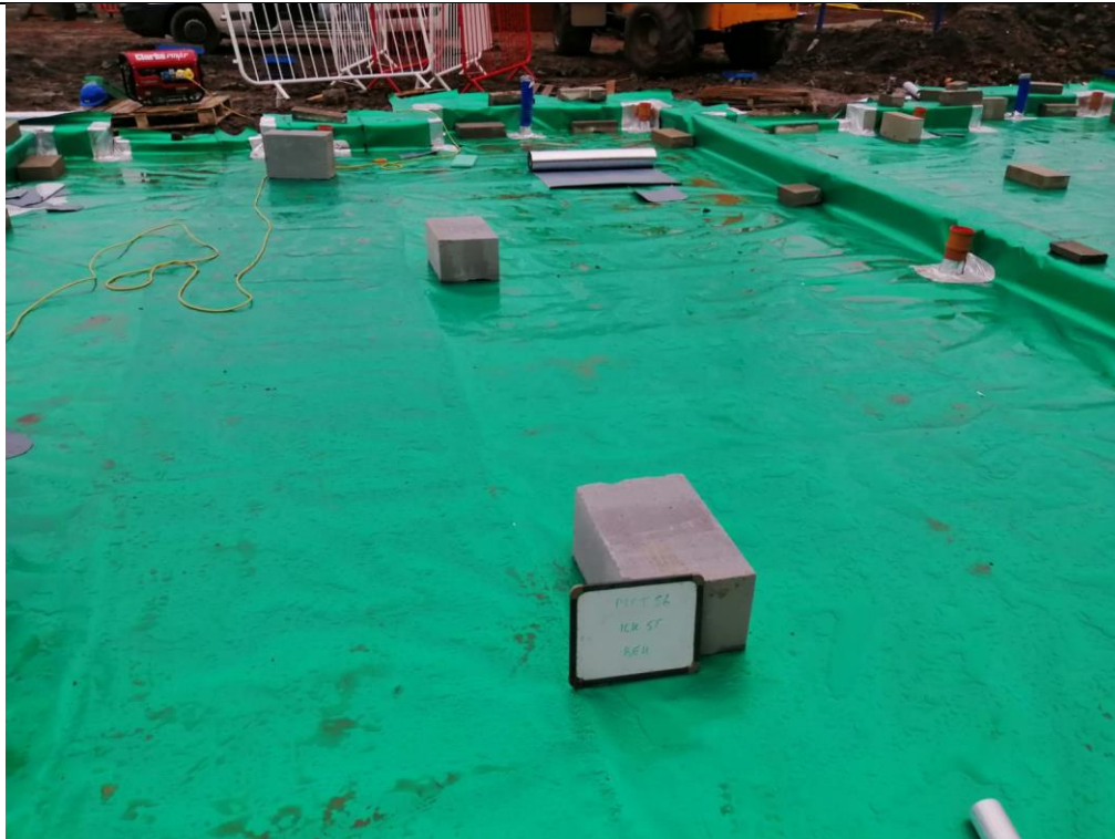
Photograph 7: Validation of Gas Membrane Installation
