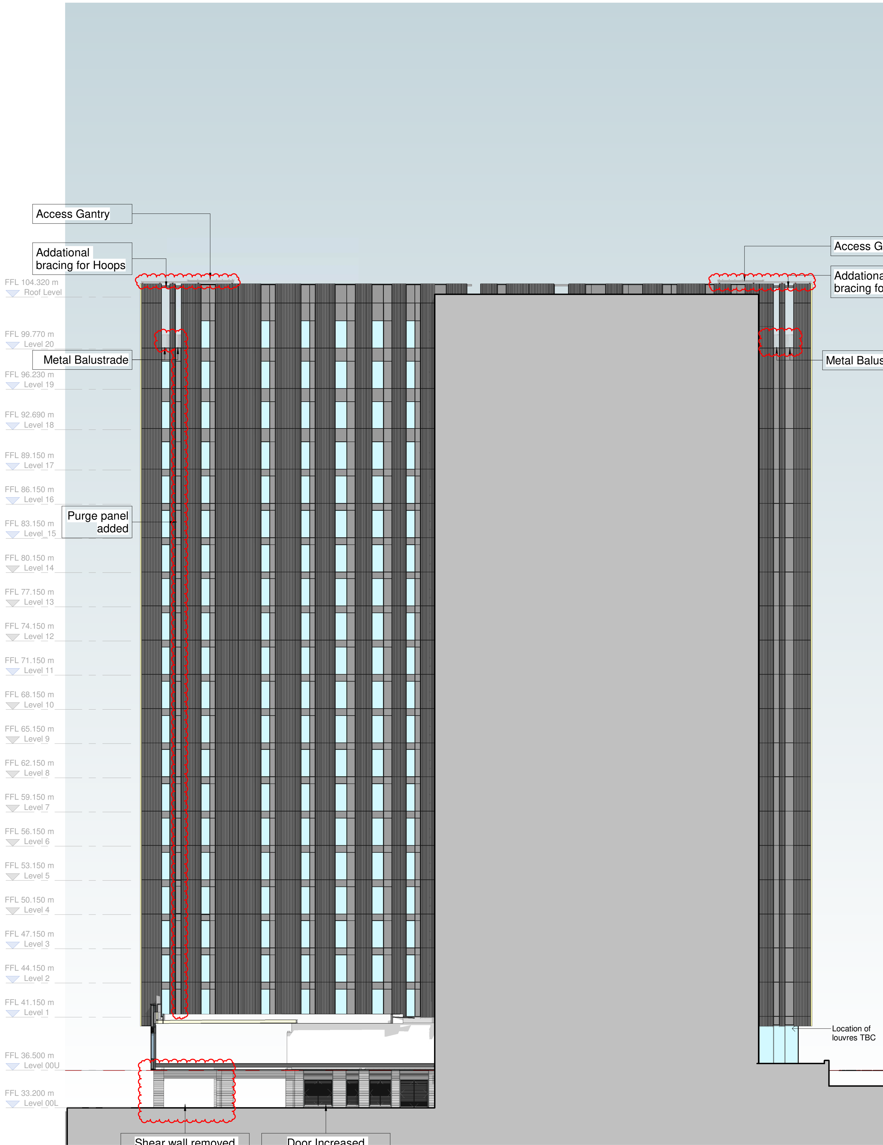
Section CC
