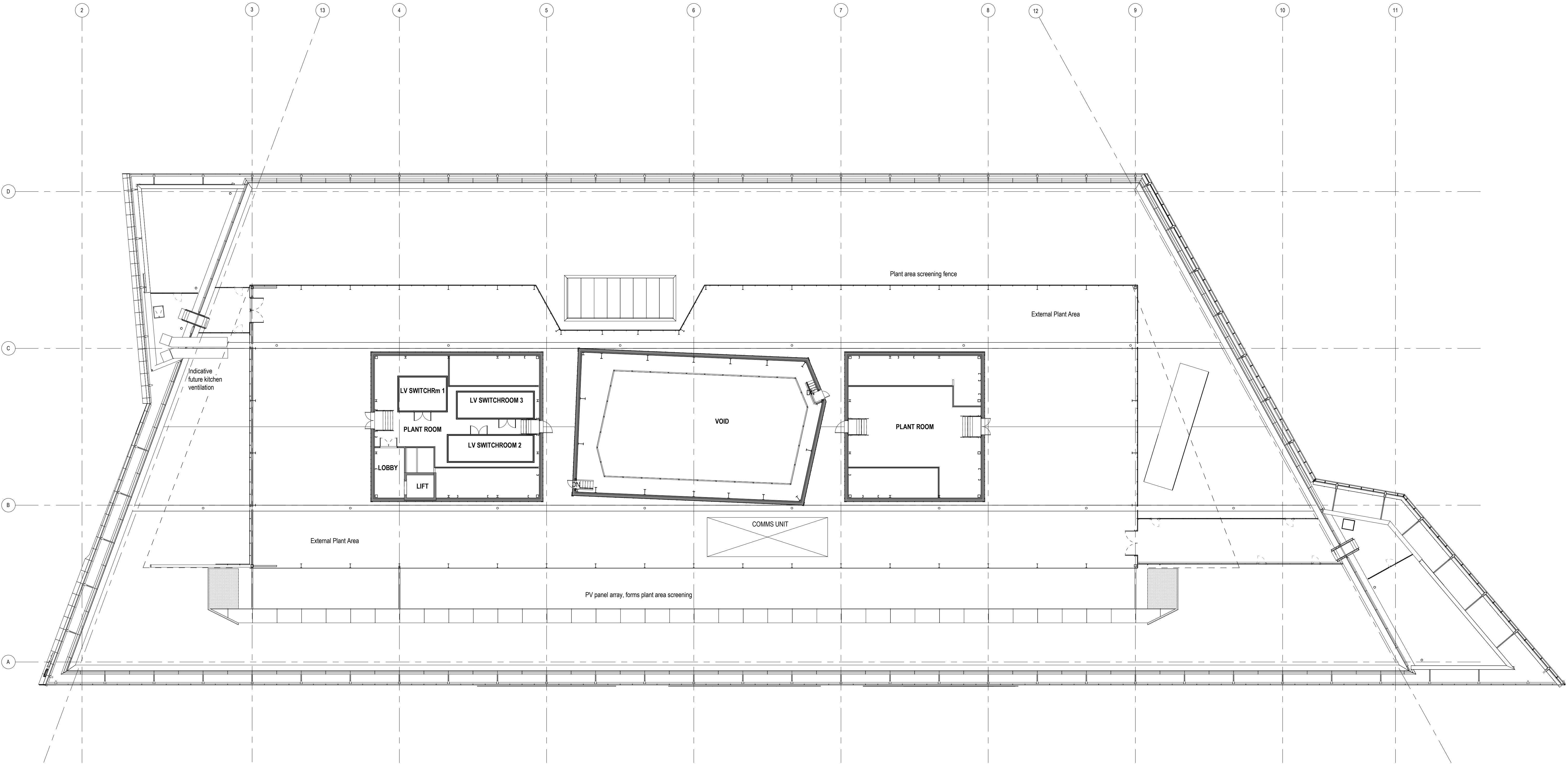
1 GA Plan - Phase 1 - Plant Layout 1 : 200
