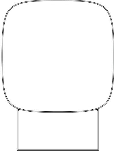
TYPICAL INTERNAL FRAME NTS (370mm (h) = 3mm thick - 445mm (h) and above = 5mm thick)
