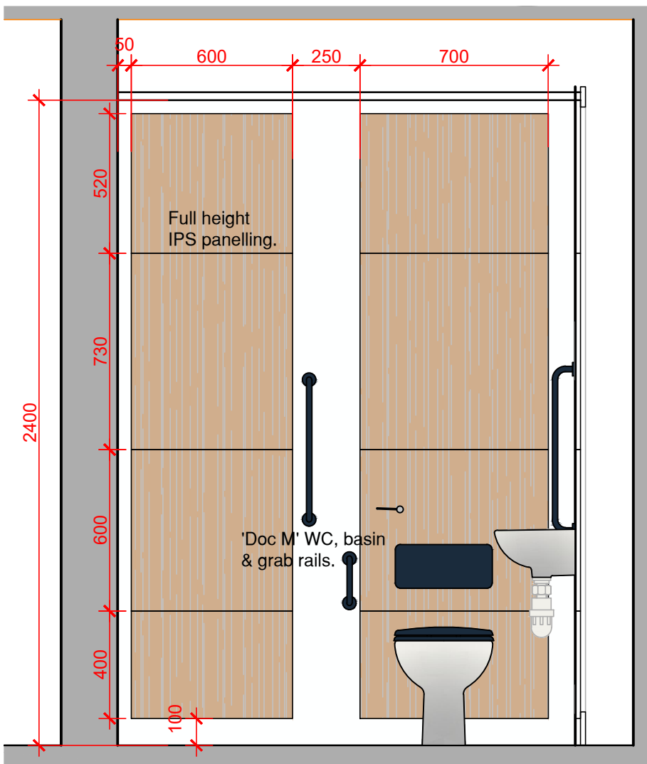
ELEVATION A Scale 1:20
