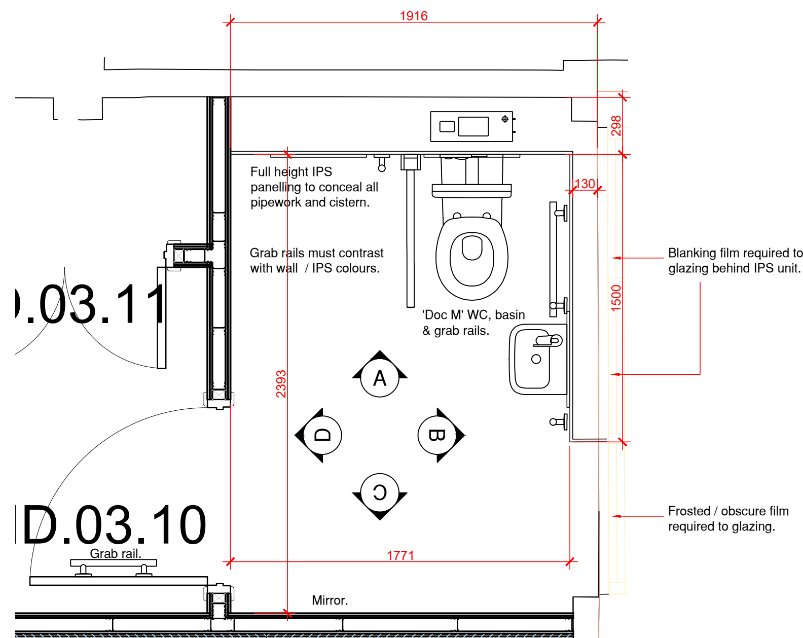
PLAN Scale 1:20
