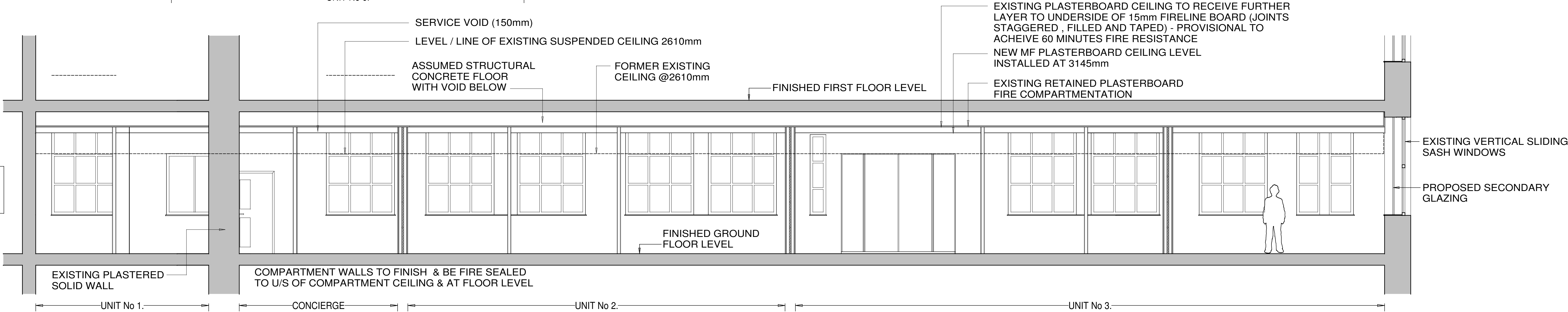
PROPOSED SECTION D-D
