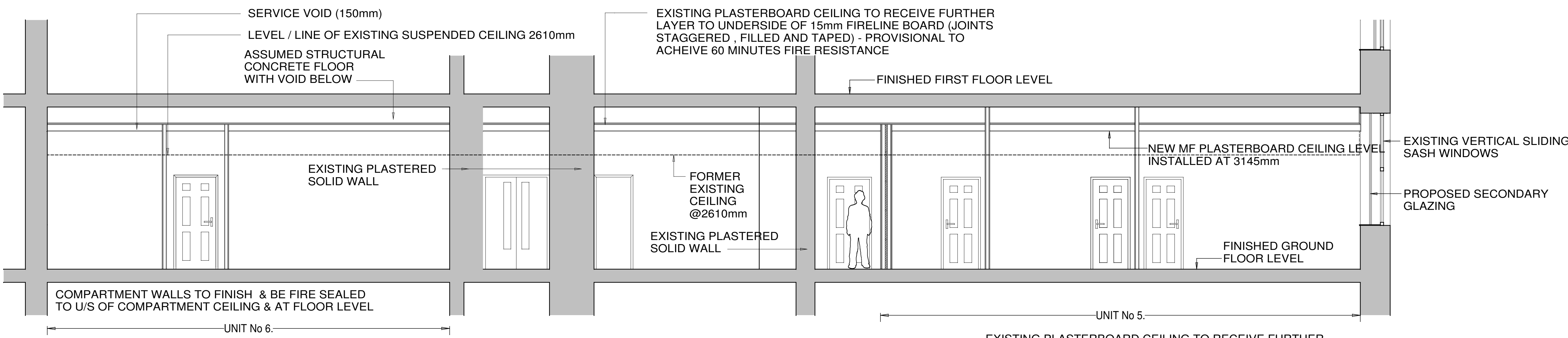
PROPOSED SECTION C-C
