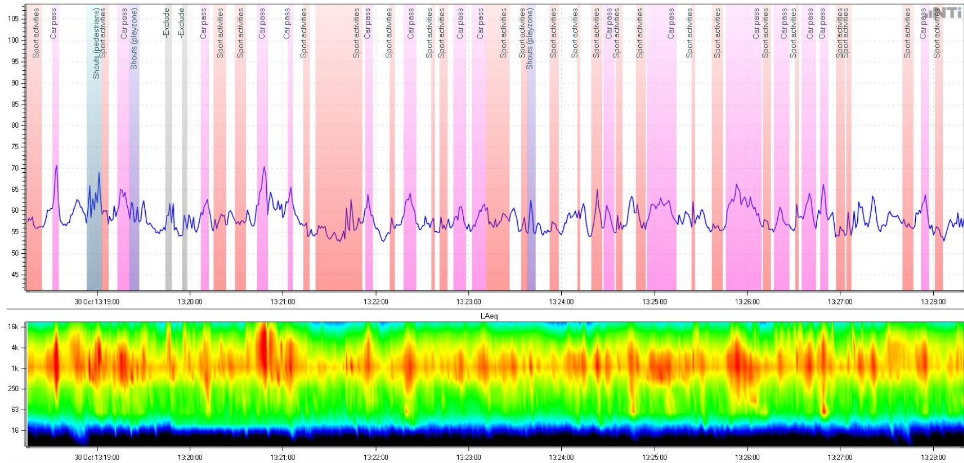
Figure 5 The time history of L_{Aeq,T} of 10-min ambient noise levels measurements at P1
