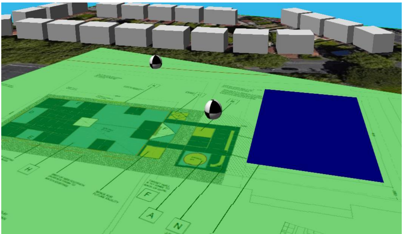
Figure 8 3D view of the CadnaA model
