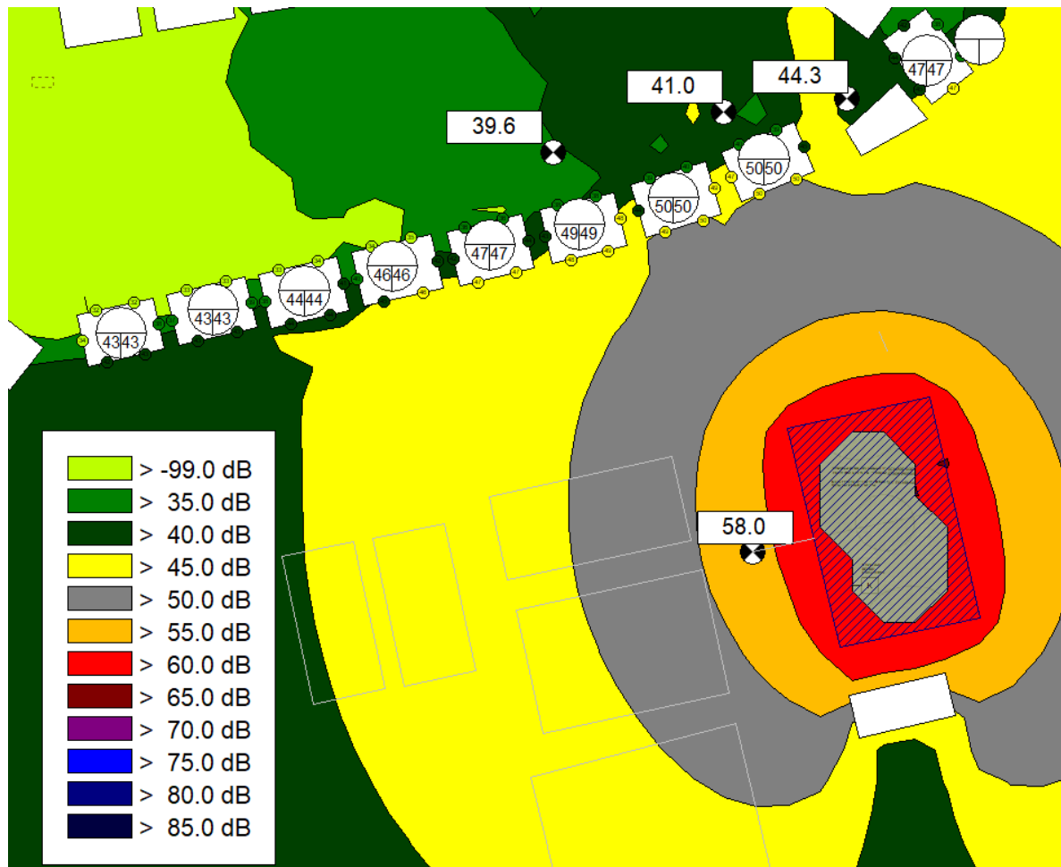
Figure 9 Small sided pitch activities noise impact levels calculated at the facades and within the gardens
