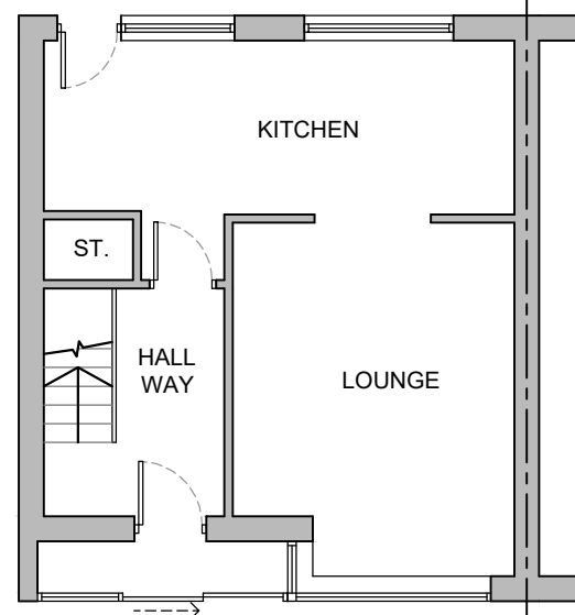
GROUND FLOOR 1:100
