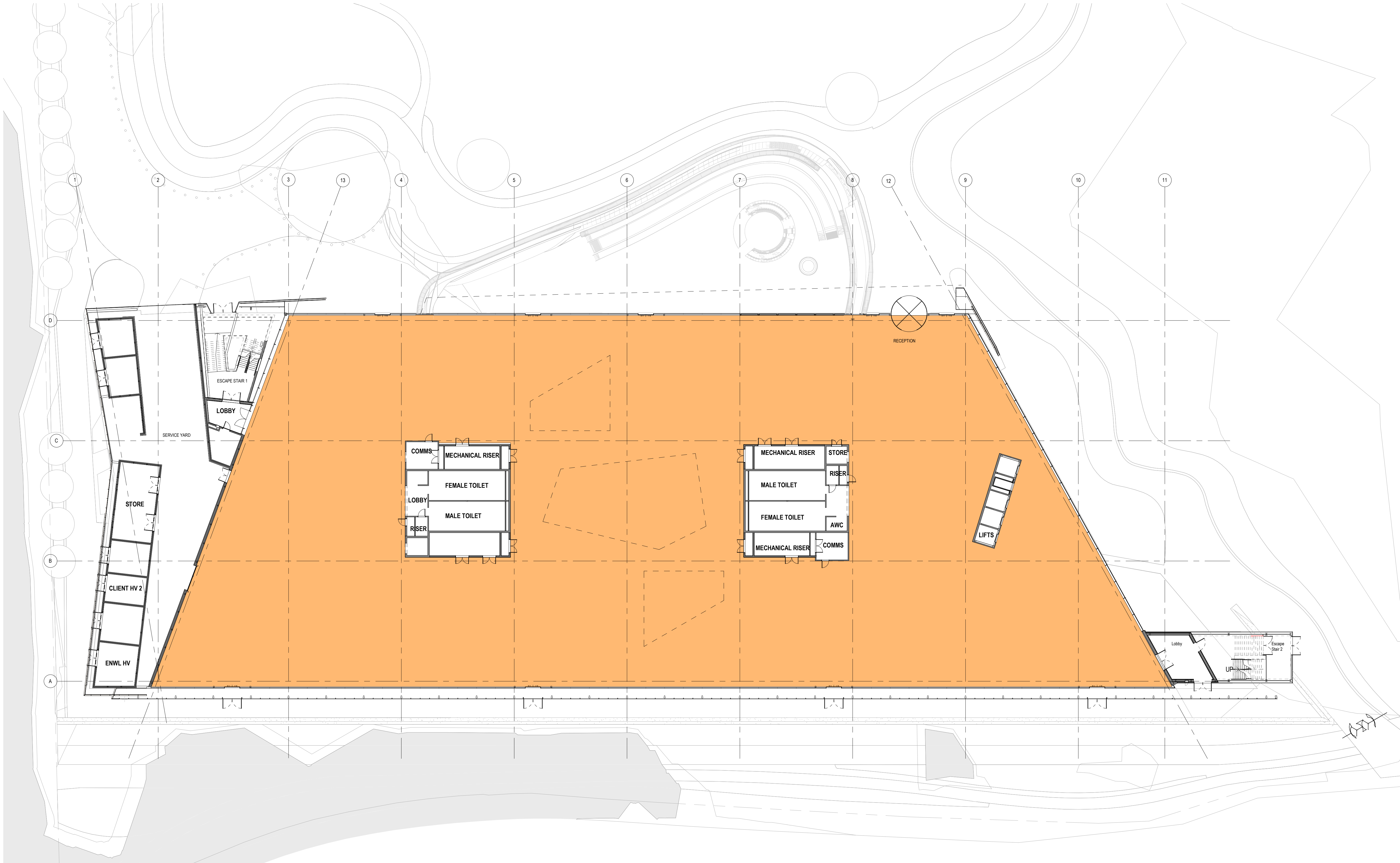
1 GA Plan - Phase 1 - Ground Floor Layout in Context 1 : 250
