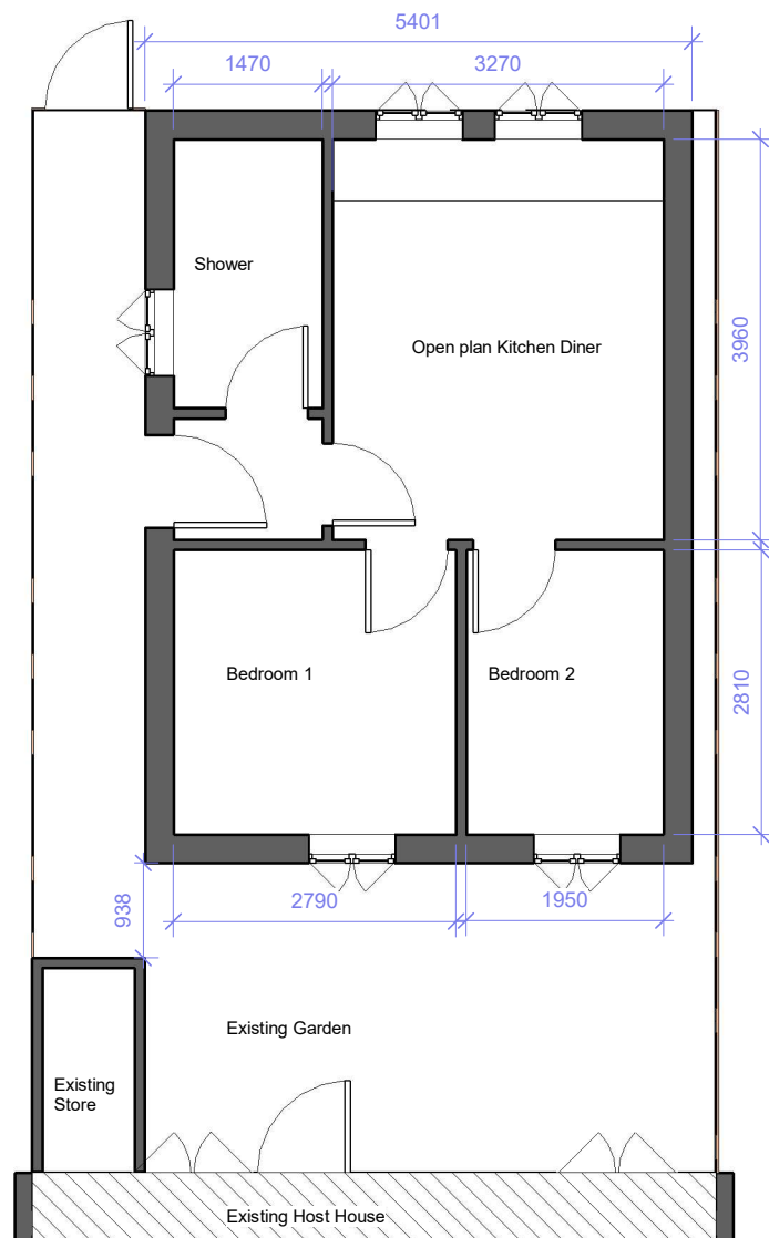
1 00 Ground Floor 1 : 50
