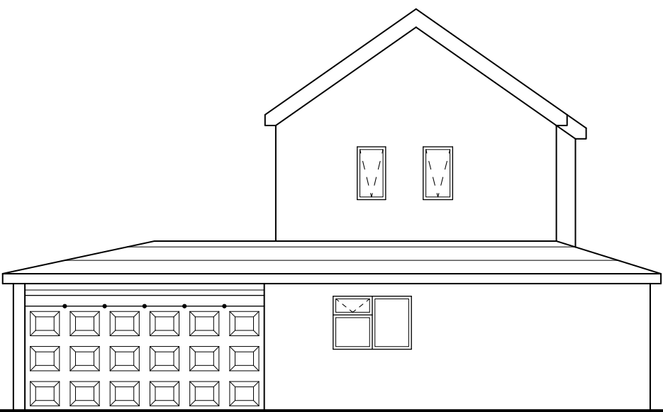
NORTH EAST ELEVATION SCALE 1:100 EXISTING - E006
