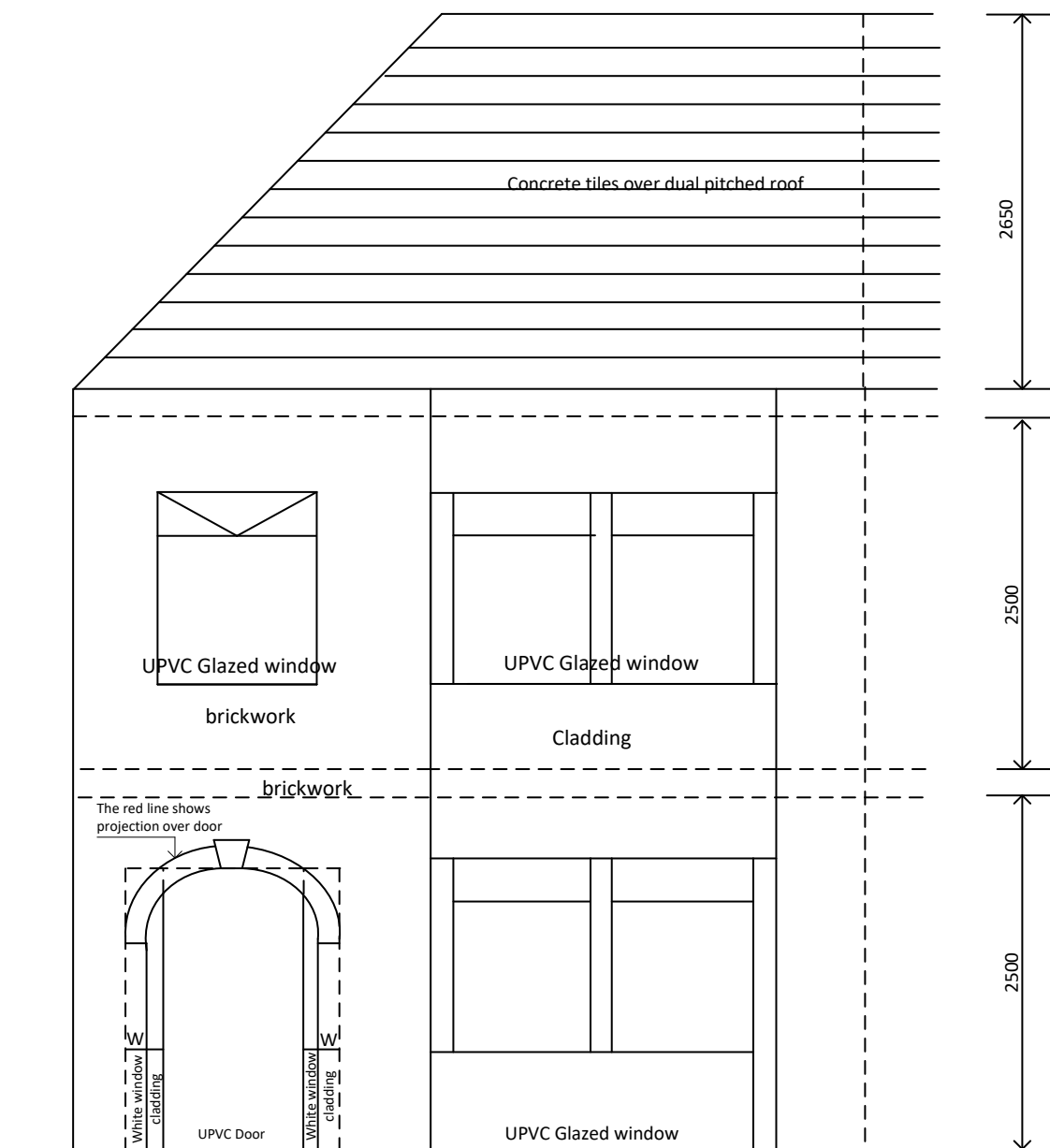
EXISTING FRONT ELEVATIONS
