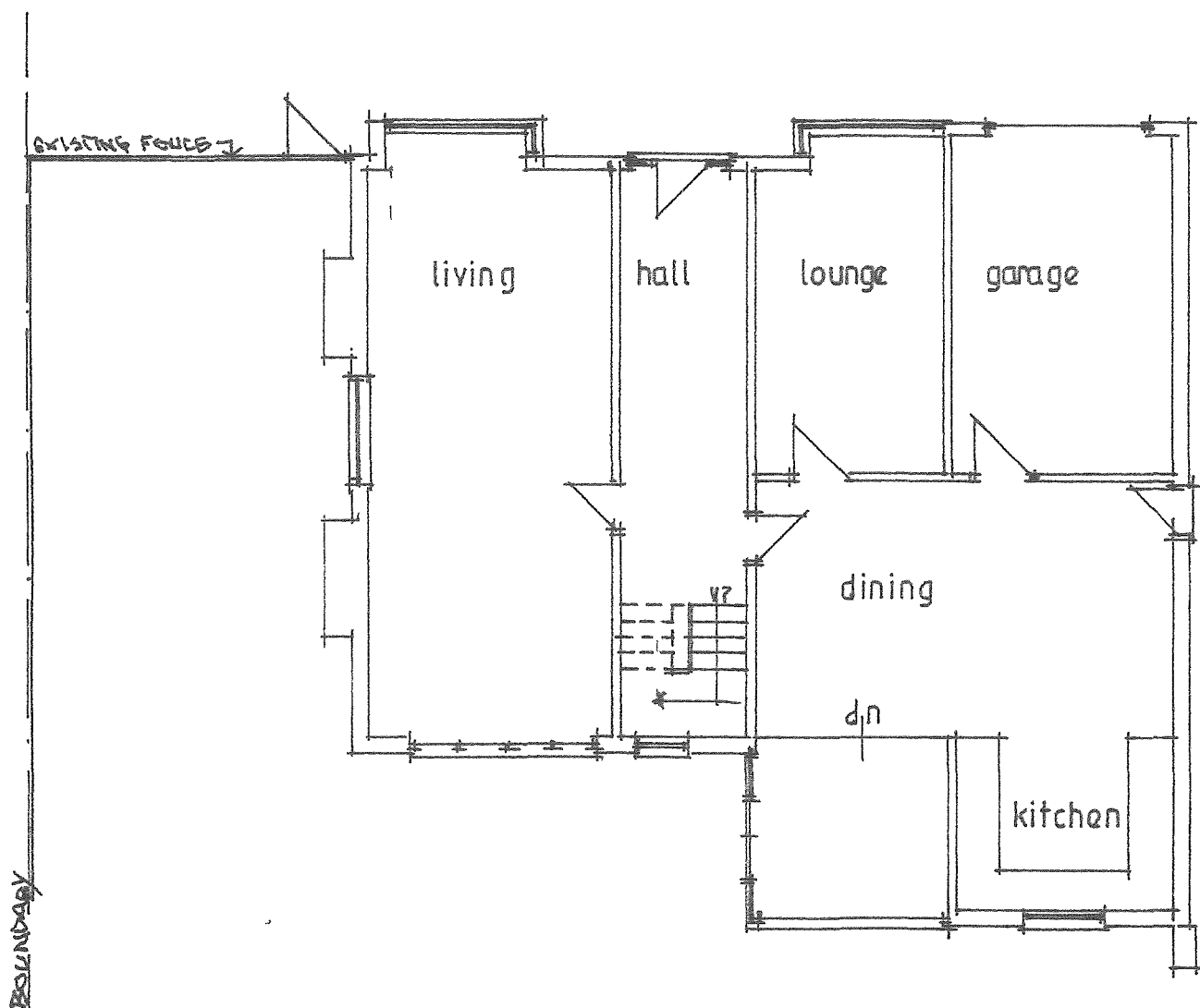
GROUND FLOOR
