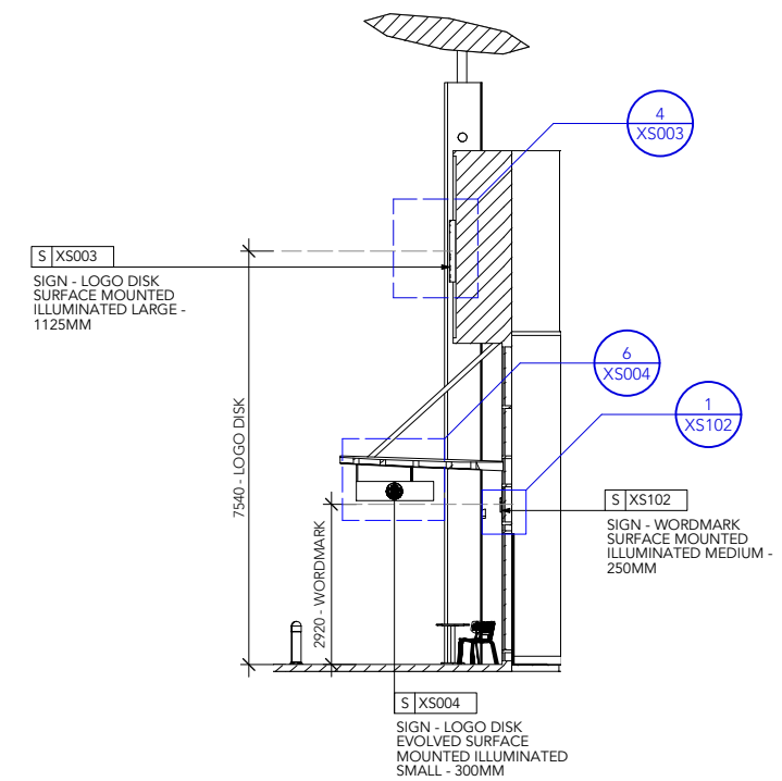
8 SIGNAGE DETAIL OVERVIEW
