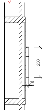
2 XS102 - SIDE ELEVATION 1:20
