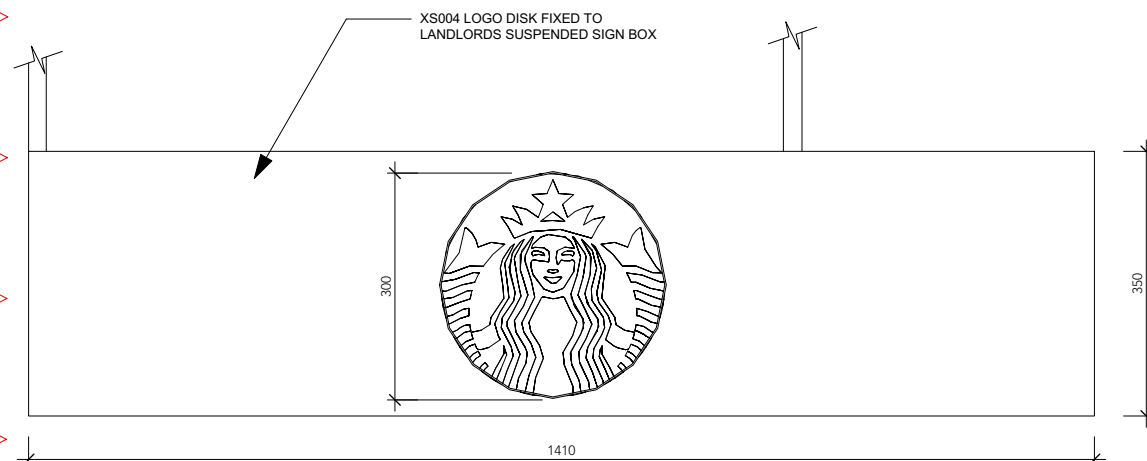
6 ID XS004 - LOGO DISK EVOLVED SURFACE MOUNTED ILLUM. SMALL 1:10
