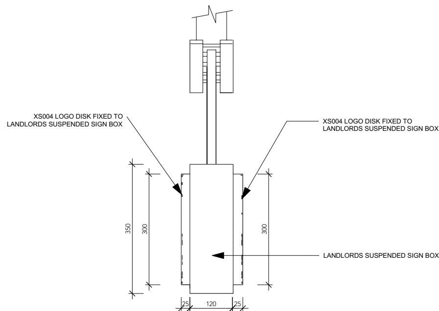
7 ID XS004 - LOGO DISKS - END ELEVATION 1:10
