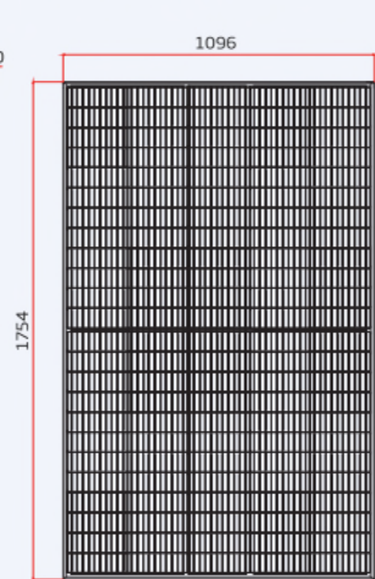
Front View
