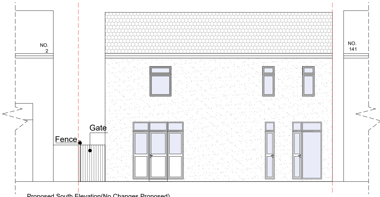
Proposed South Elevation(No Changes Proposed)
