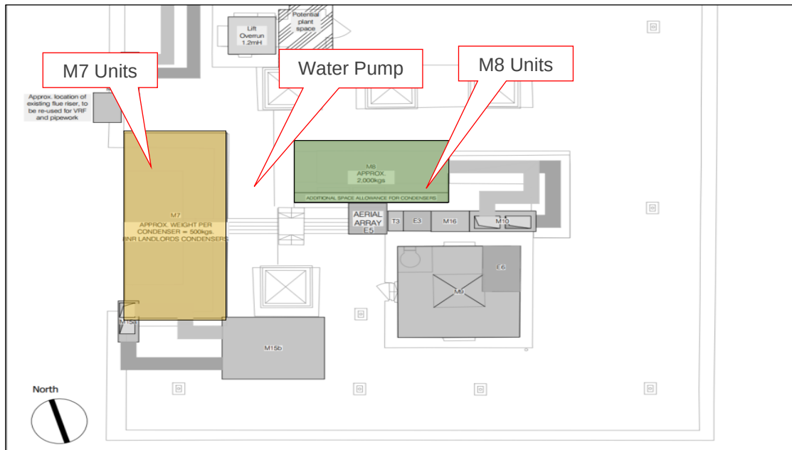
Proposed plant location on roof
