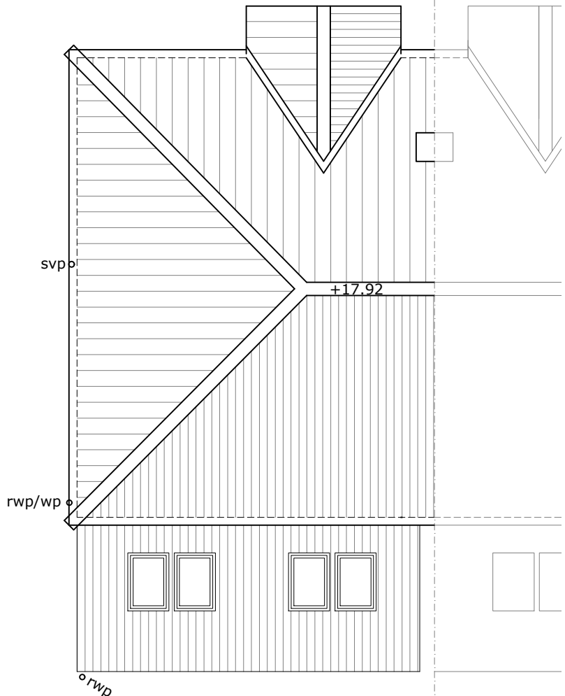
ROOF PLAN
