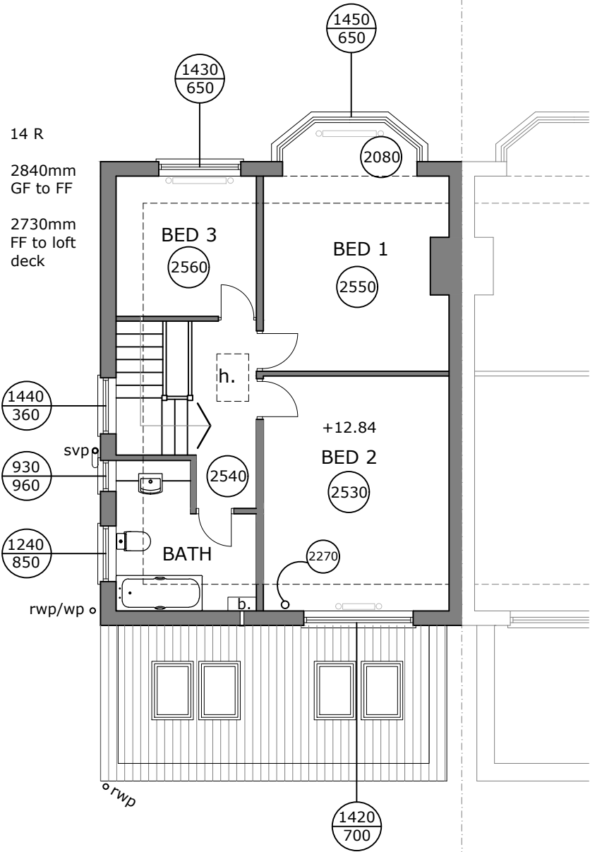
FIRST FLOOR
