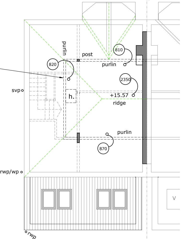
ATTIC PLAN
