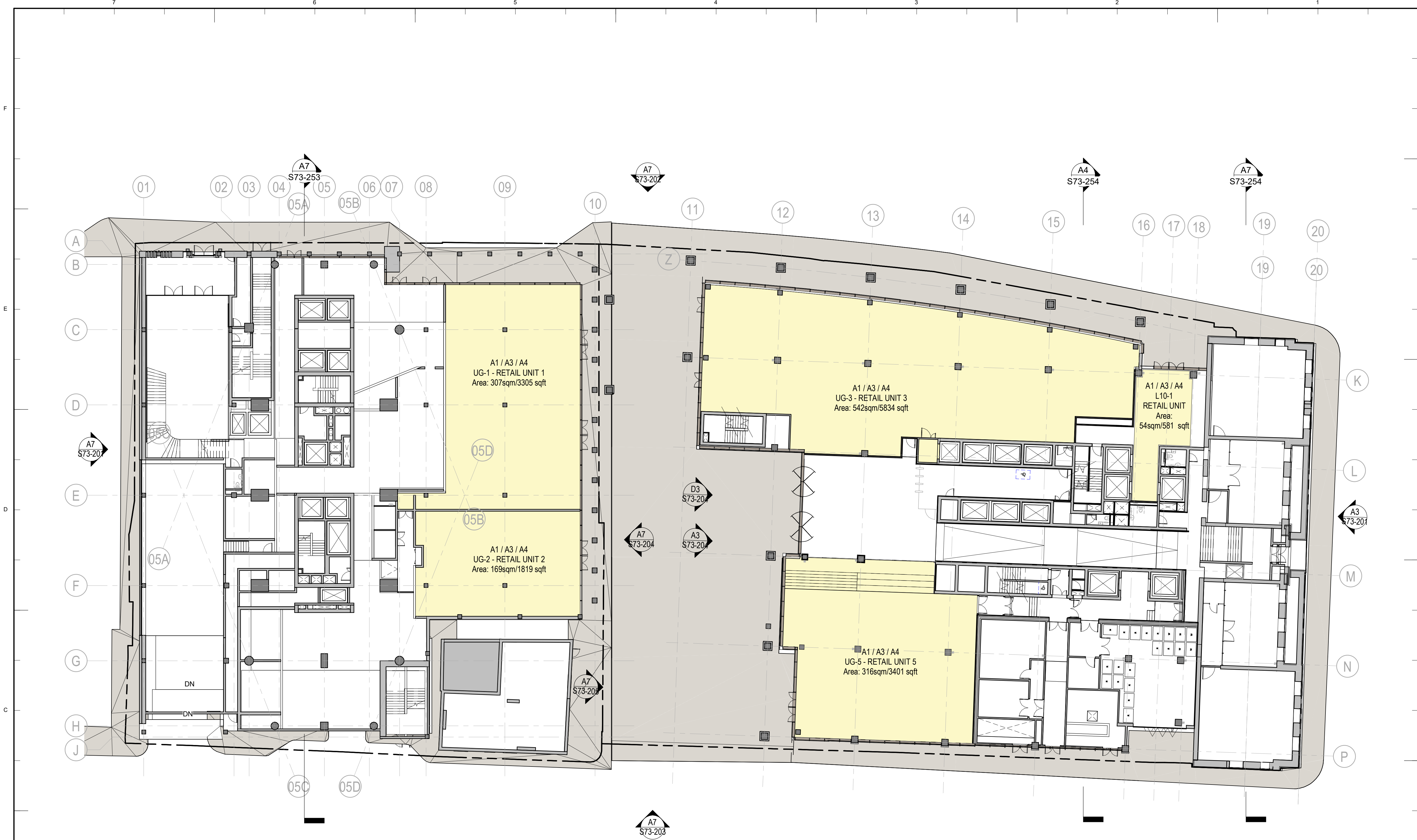
1 RETAIL PLAN - GROUND FLOOR 1 : 200
