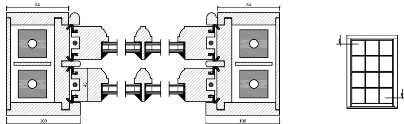
1 DETAIL PLAN HERITAGE CASEMENT WINDOW 1:5
