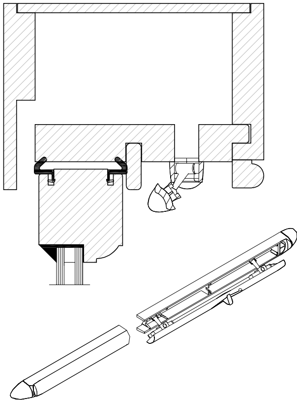
3 DETAIL TRICKLE VENT HERITAGE CASEMENT WINDOW 1:2
