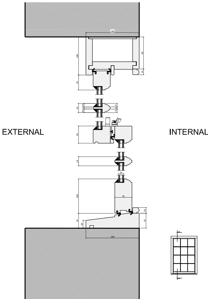
2 DETAIL SECTION HERITAGE CASEMENT WINDOW 1:5
