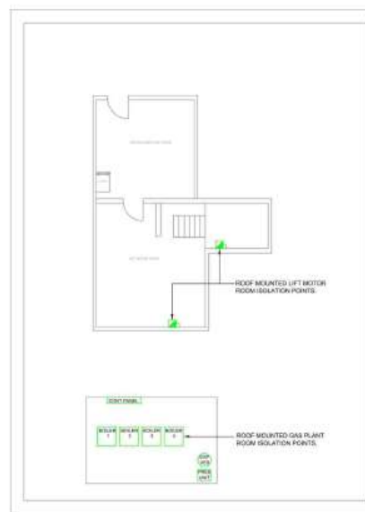
ROOF LAYOUT
