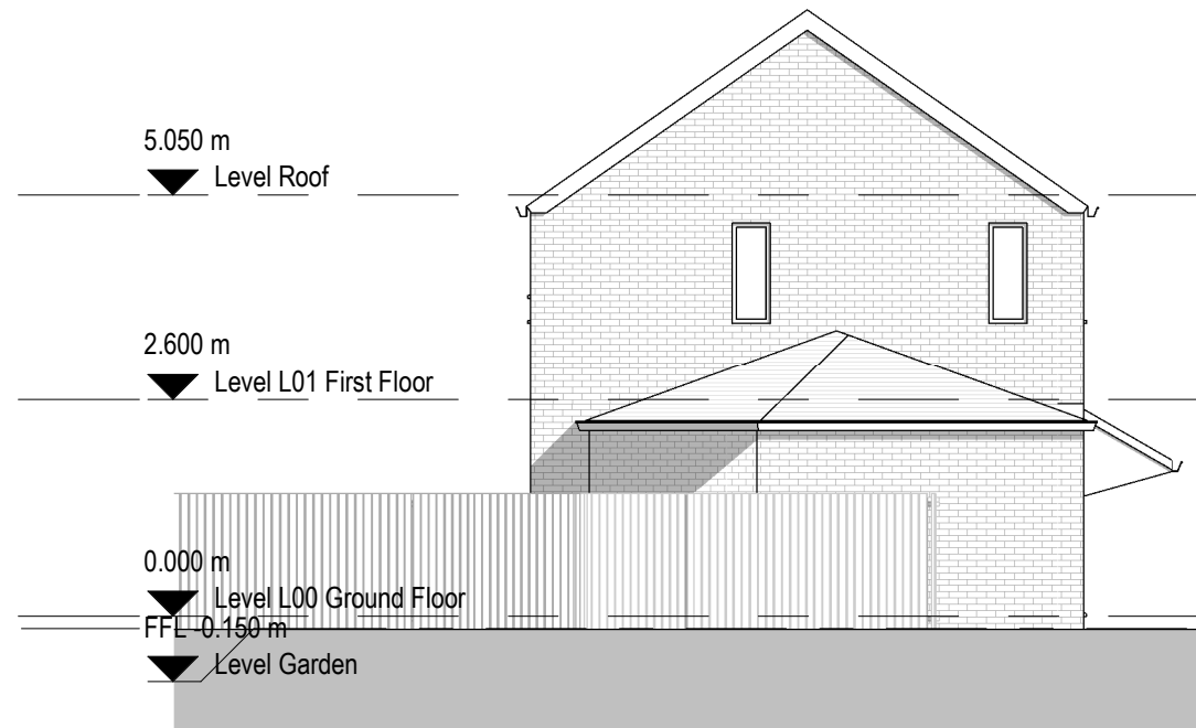
2 Existing West Elevation 1 : 100
