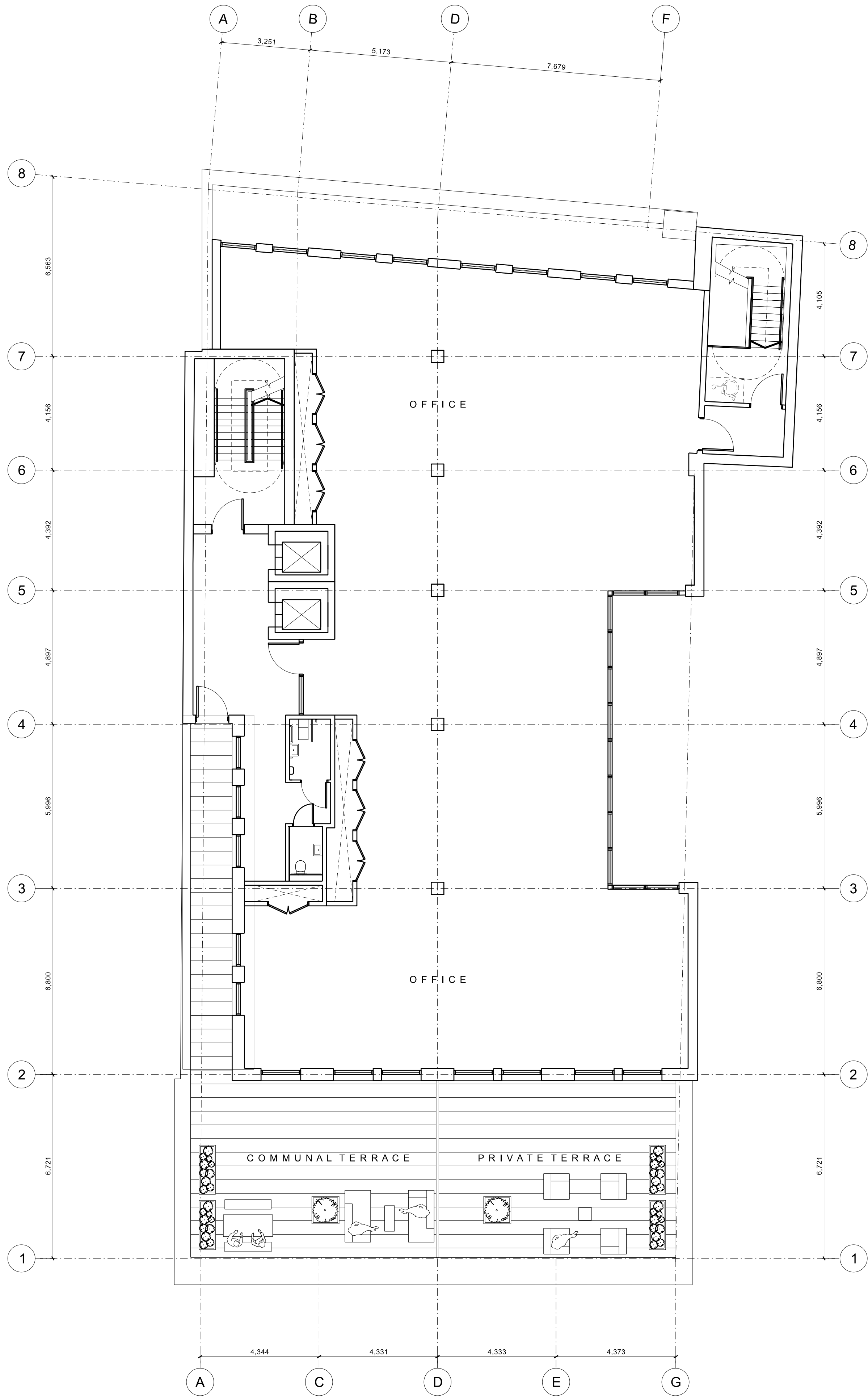
LEVEL 06
