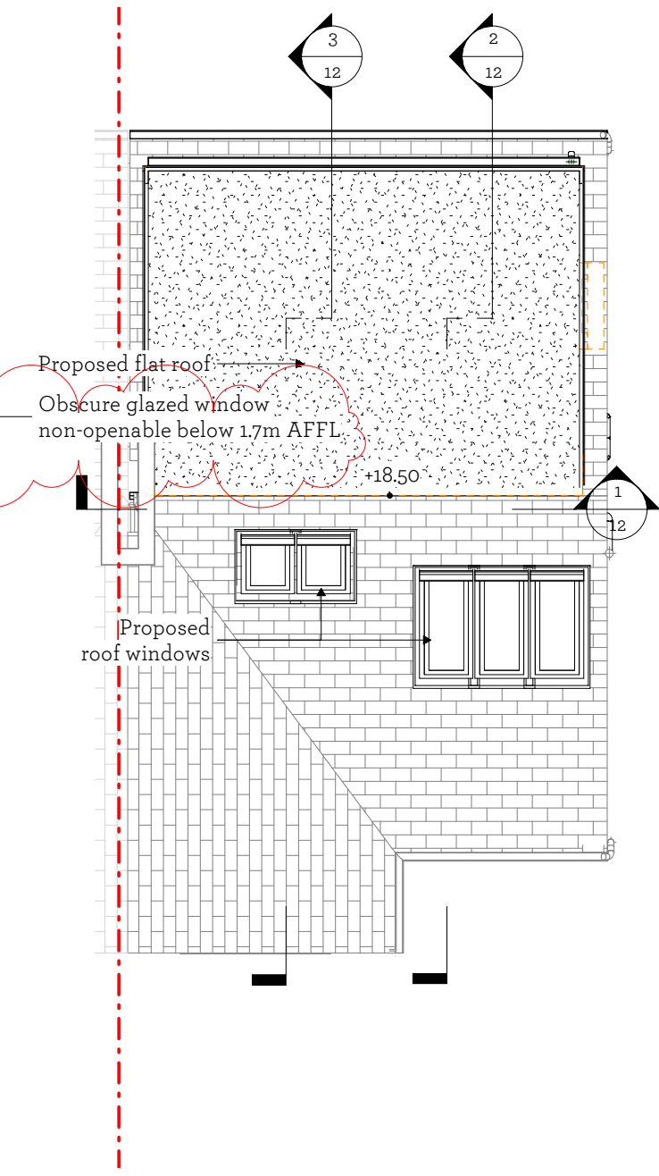
Proposed Roof 1 : 100
