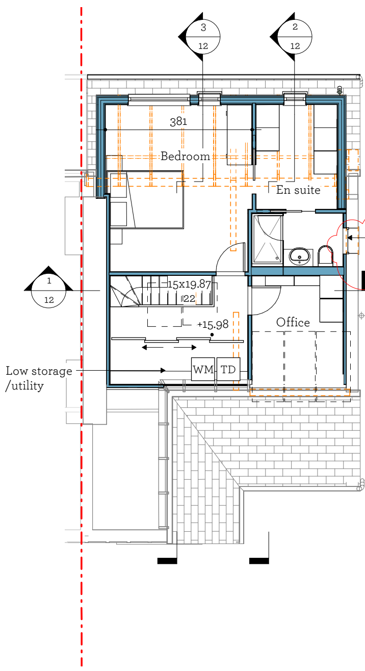
Proposed Loft 1 : 100
