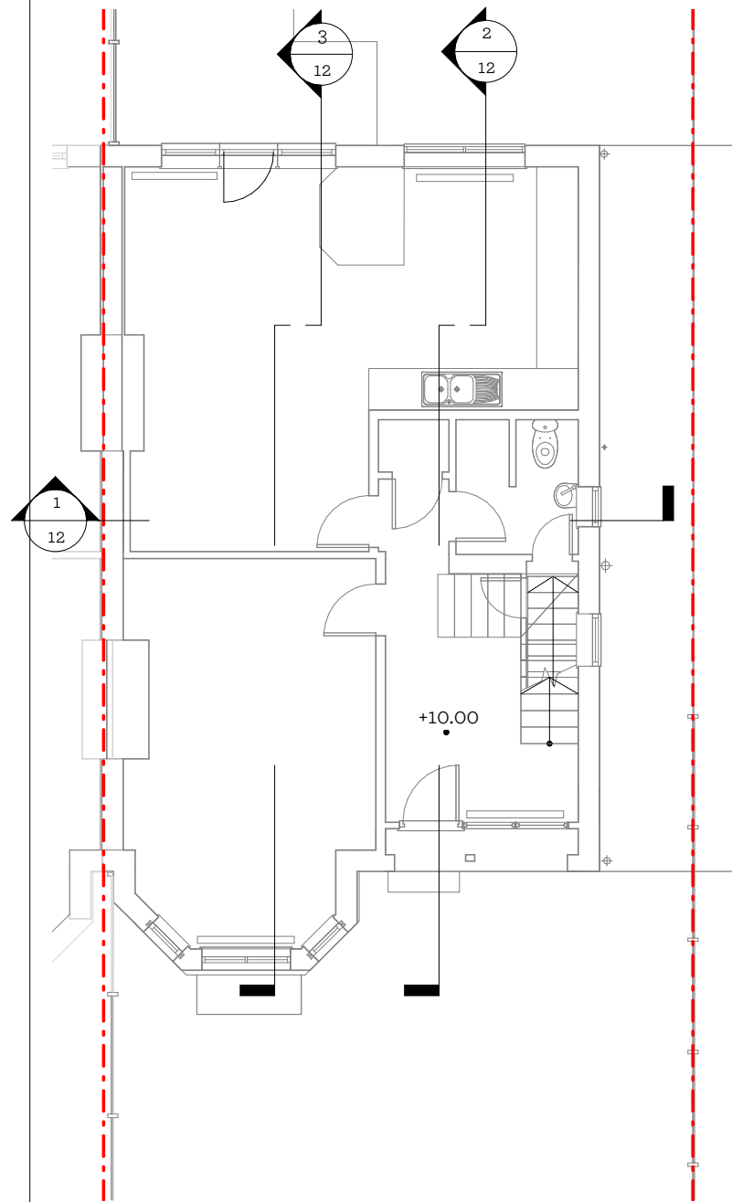
Proposed Ground Floor 1 : 100
