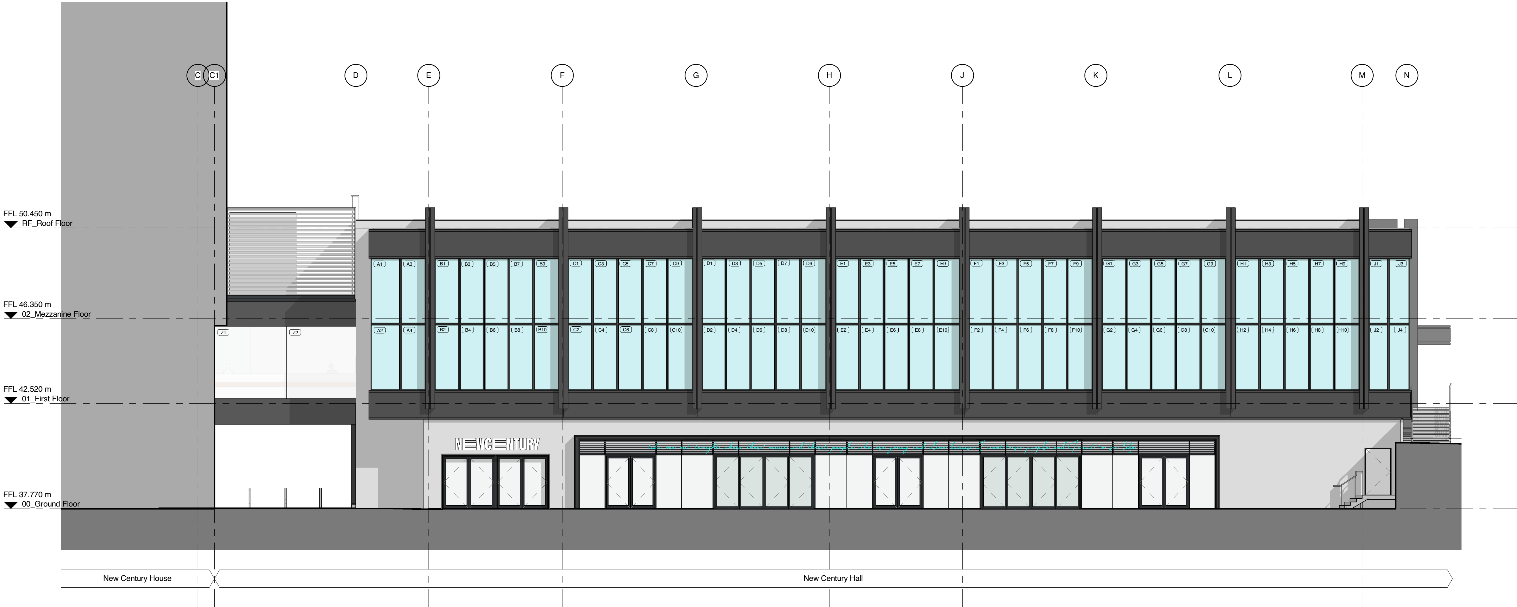
1 20225 GA South Elevation - Mayes Street 1 : 100
