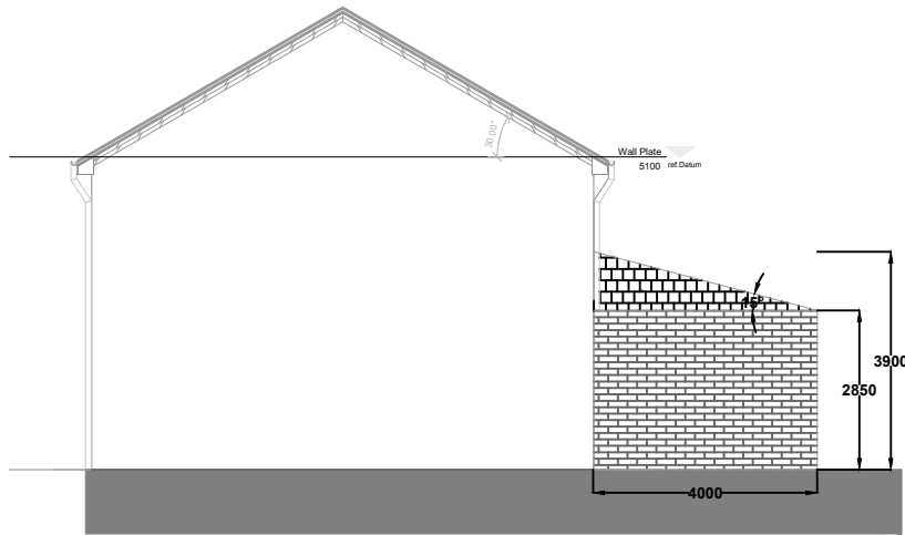
PROPOSED SIDE B ELEVATION
