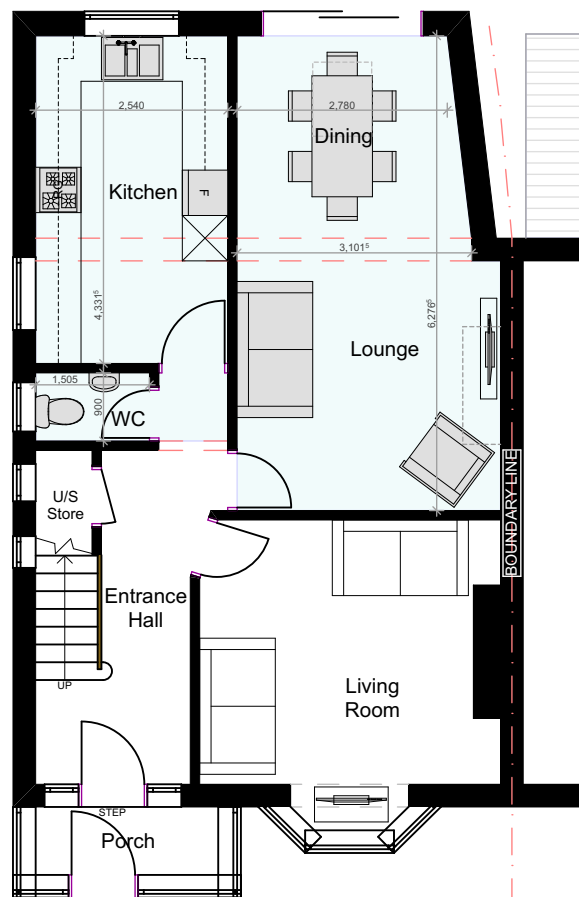
PROPOSED GA GROUND FLOOR PLAN
