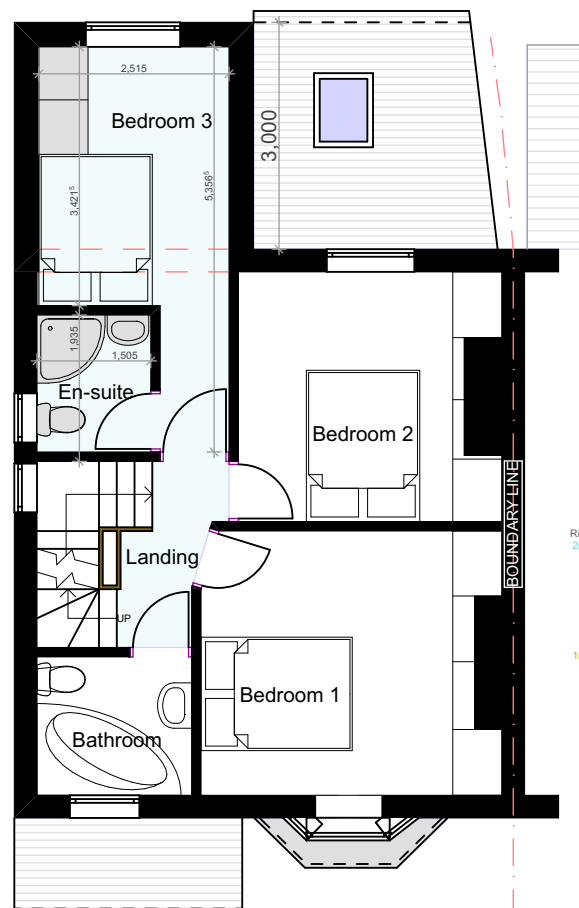
PROPOSED GA FIRST FLOOR PLAN
