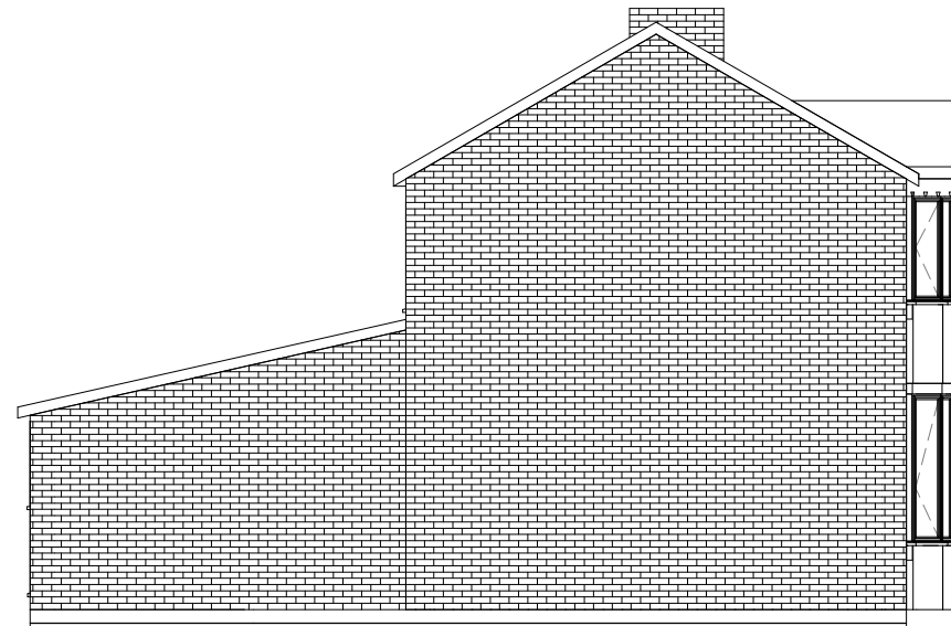
2 Left Proposed 1 : 100
