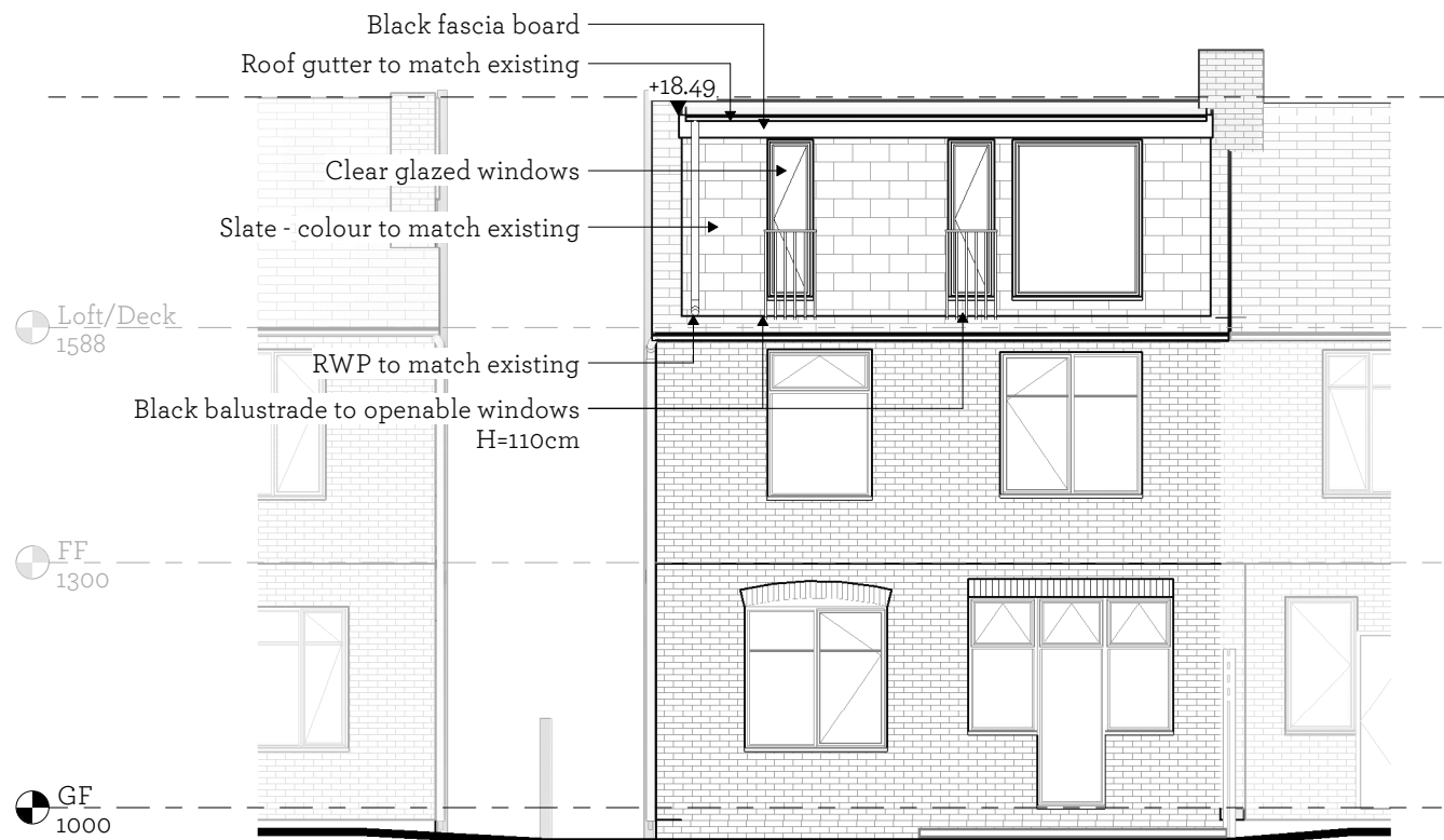
Proposed elevation West
