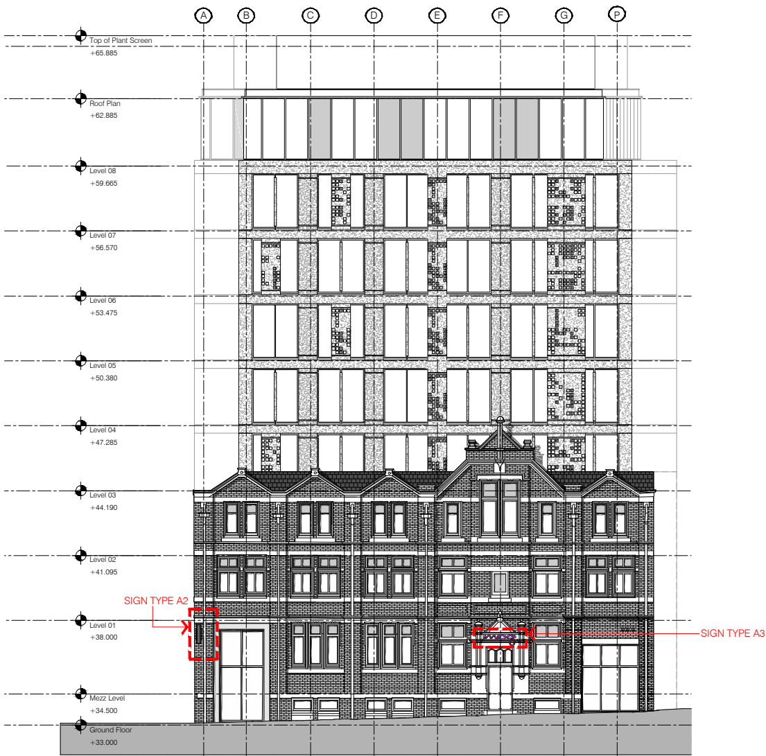
Scott Place Elevation Scale: 1:250
