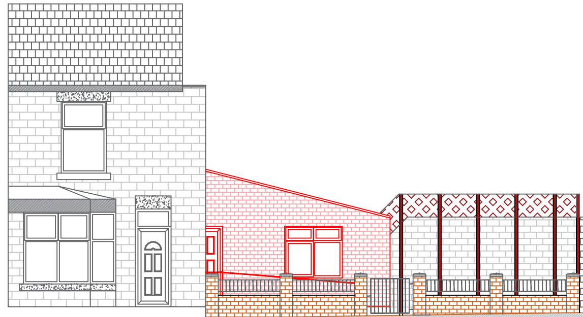
Proposed Front Fence Layout
