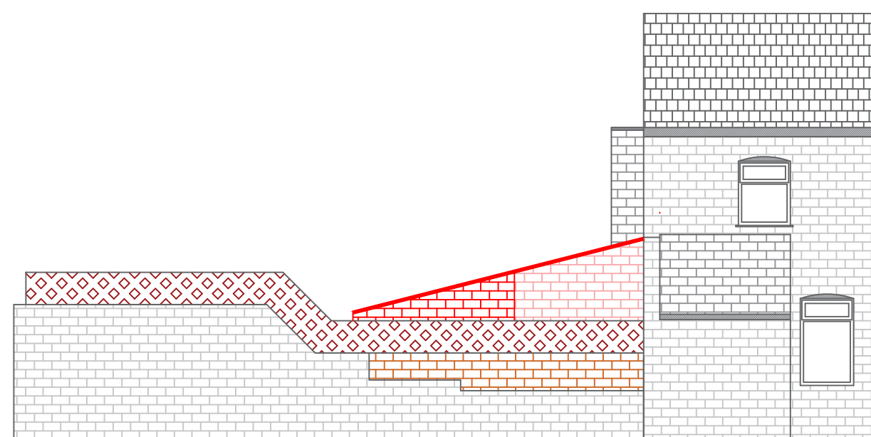
Proposed Rear boundary wall Layout
