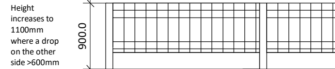
F2 900-1100mm high close boarded concrete post and TSW panel fence to have gravel board at base. Security bracket to be fixed using non-ferrous timber panels to prevent removal.
