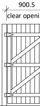
G1 Pedestrian Gate 900 x 1800mm high gate
