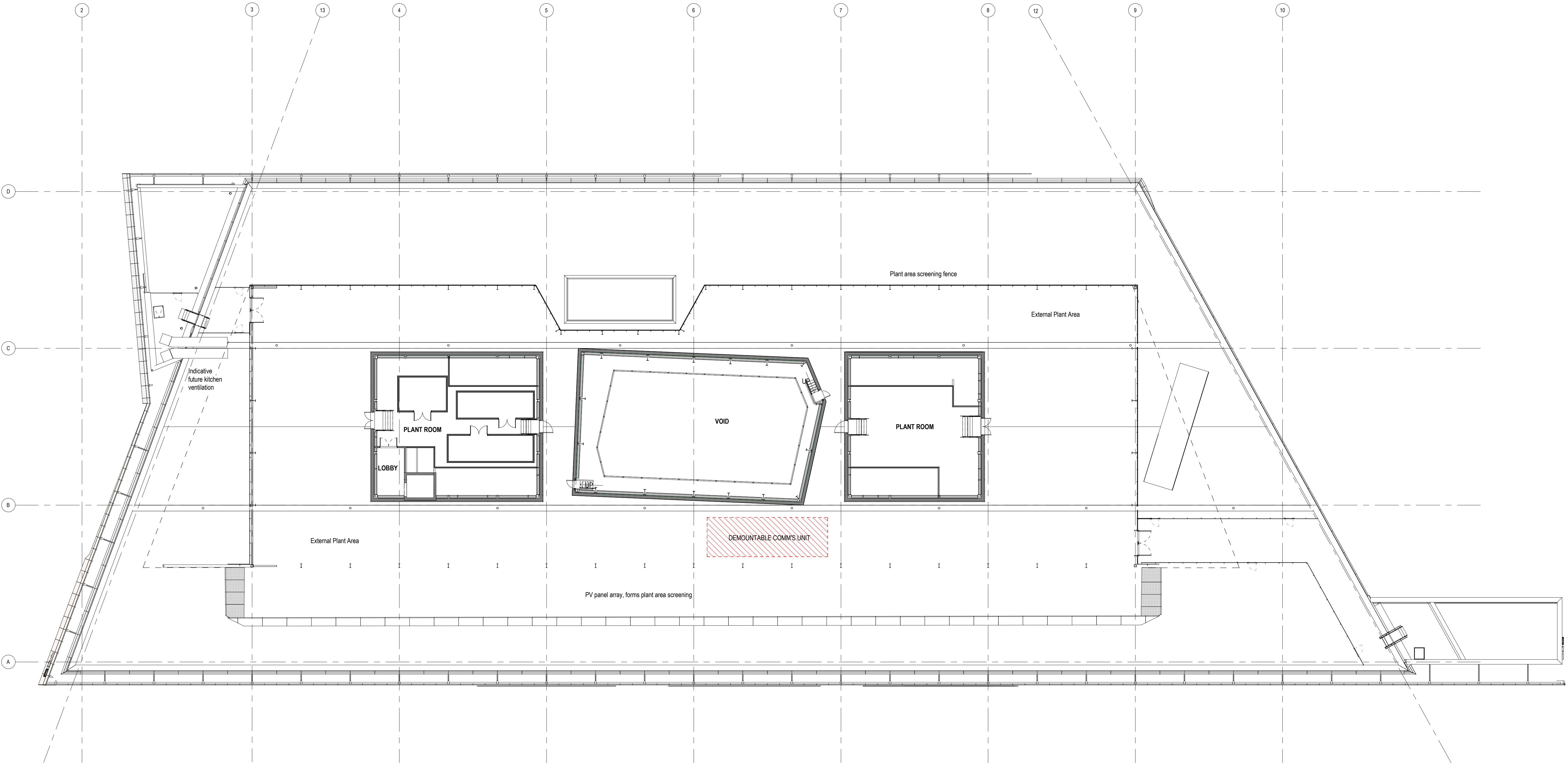
1 GA Plan - Phase 1 - Plant Layout
