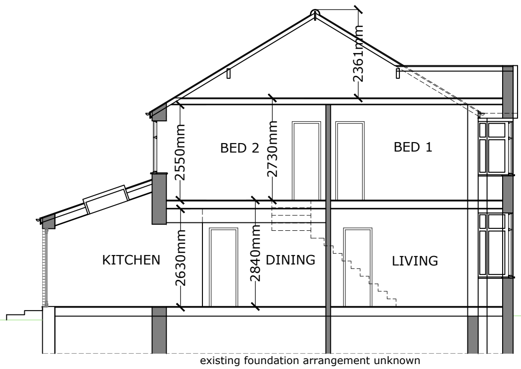
CROSS SECTION
