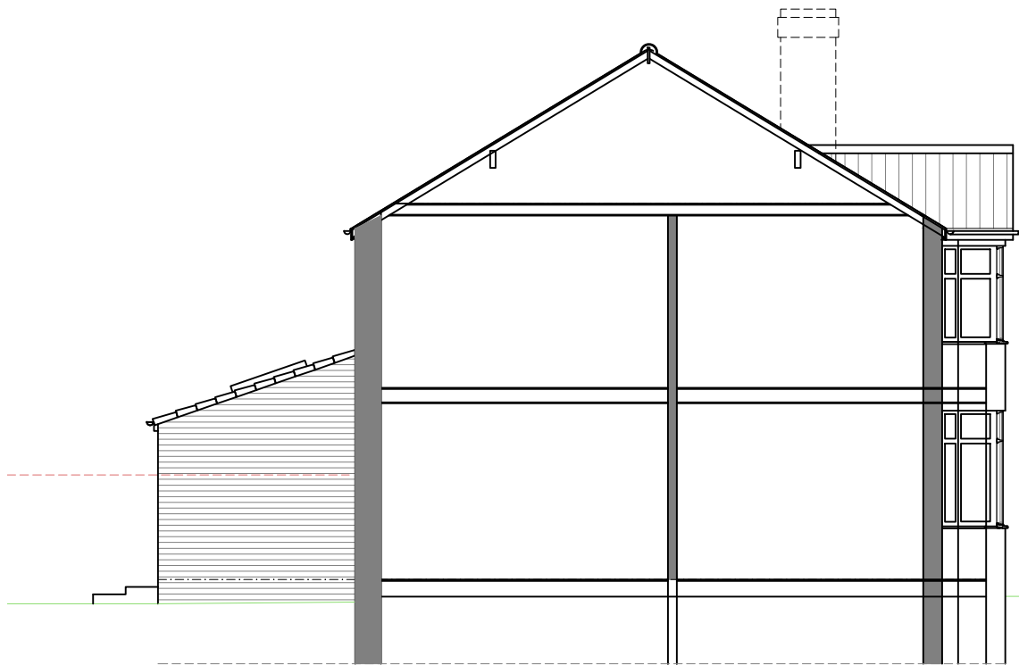
WEST ELEVATION
