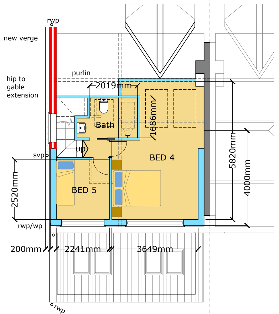
ATTIC PLAN
