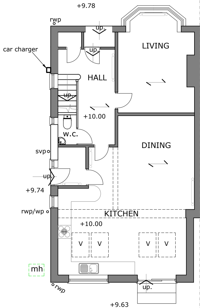
GROUND FLOOR (NO CHANGES)
