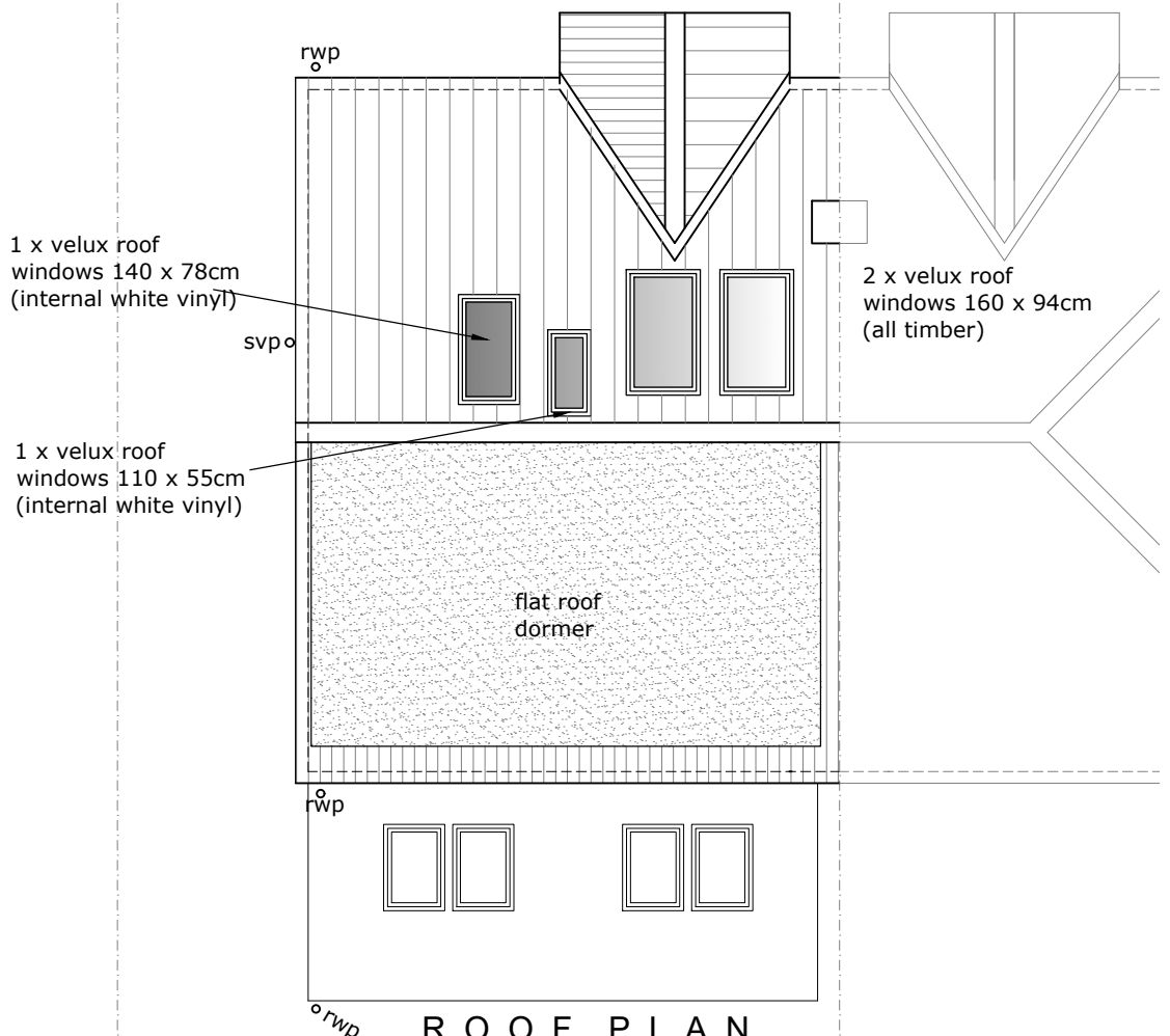
ROOF PLAN
