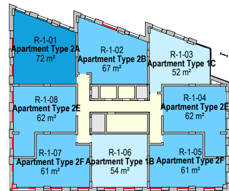
01 Room Schedule Plan - Level 01 1 : 500
