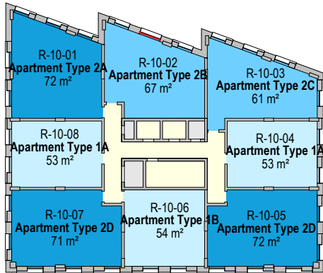
10 Room Schedule Plan - Level 10 1 : 500
