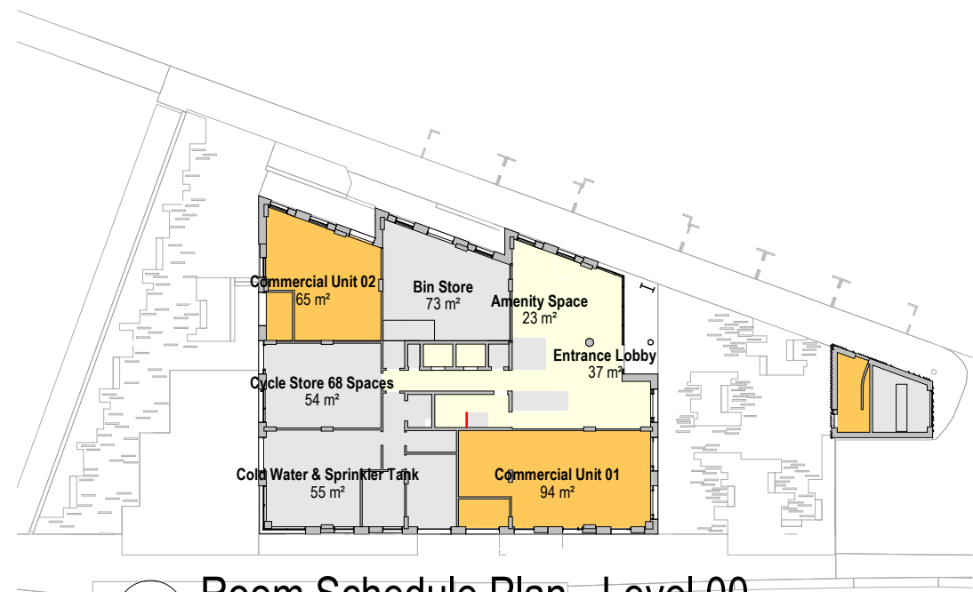
00 Room Schedule Plan - Level 00 1 : 500
