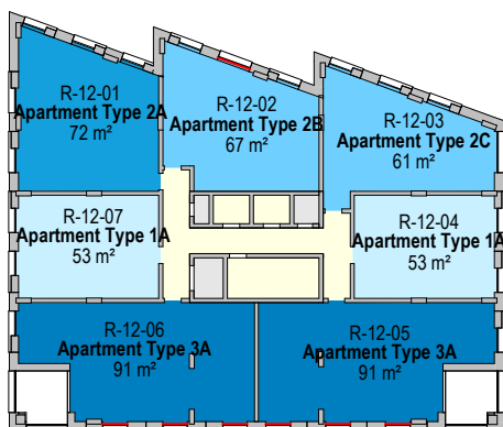
12 Room Schedule Plan - Level 12 1 : 500
