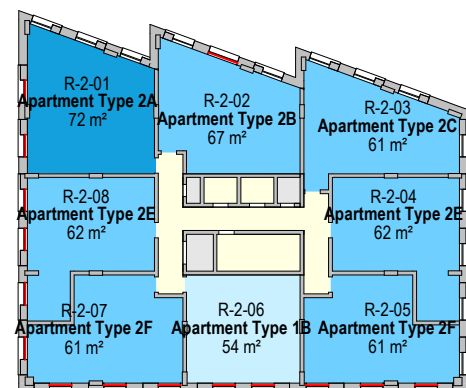
02 Room Schedule Plan - Level 02 1 : 500
