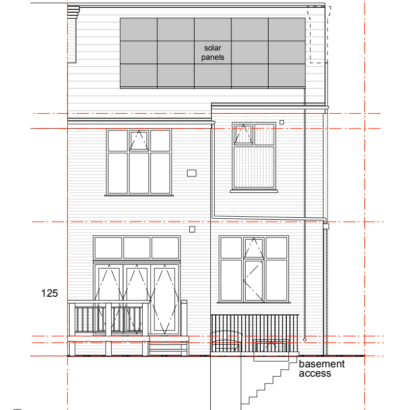
existing elevation 3
