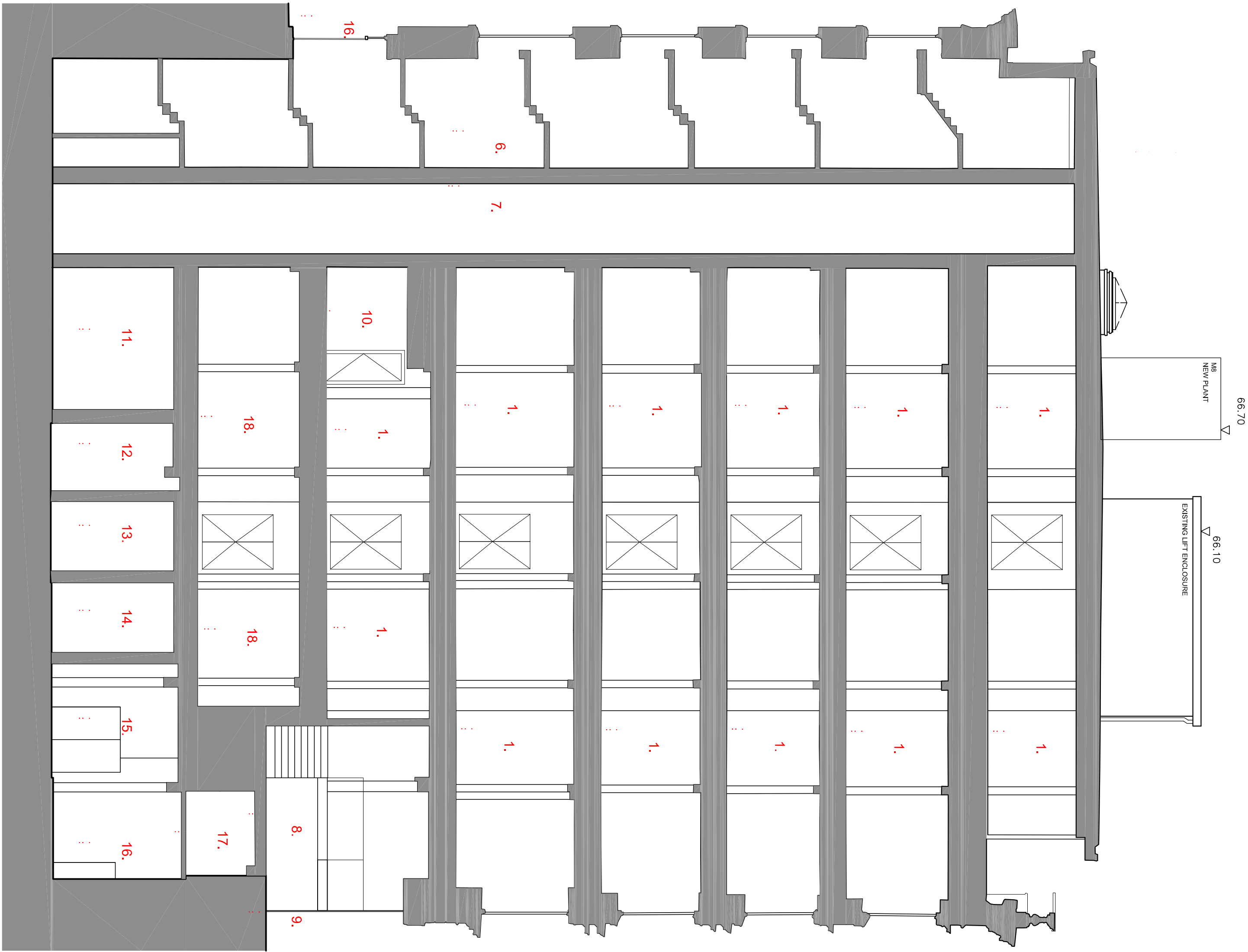
02 Section B-B'
