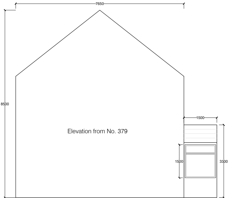
East Elevation as Existing
