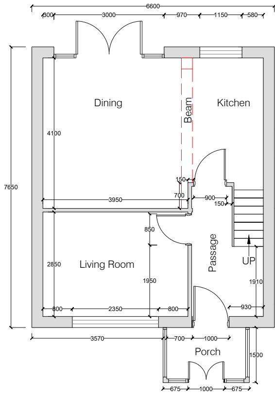
Ground Floor Plan as Existing
