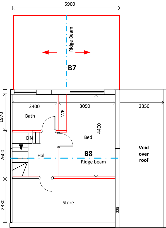
PROPOSED DORMER
