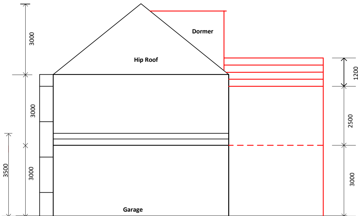
PROPOSED ELEVATION From Neighbour Side 41
