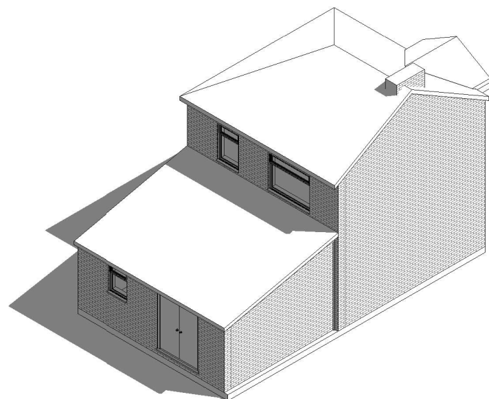
3 Rear Left Proposed
