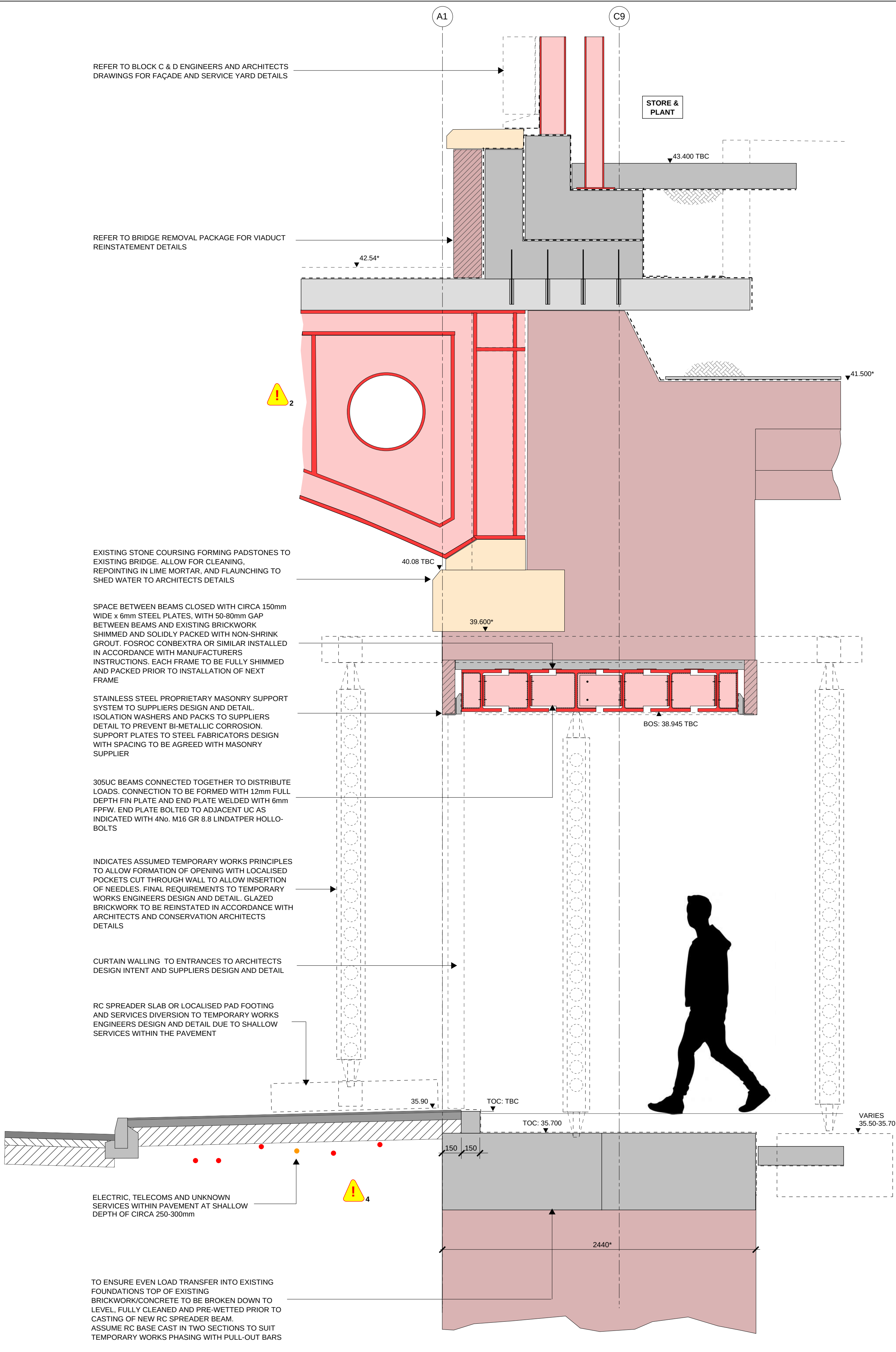
SECTION B-B 1:20
