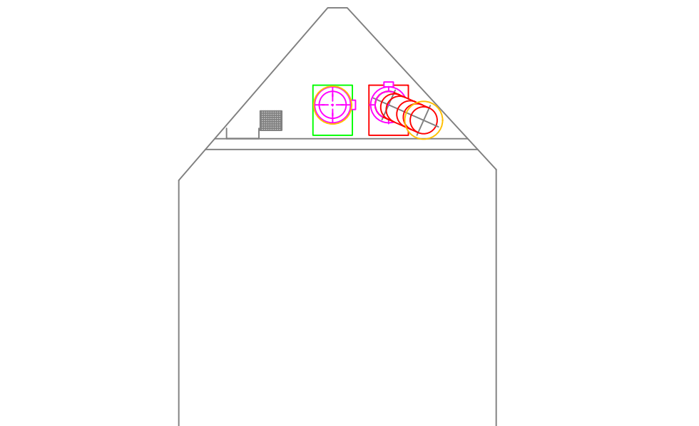
Female WC Section 1:50 @ A1
