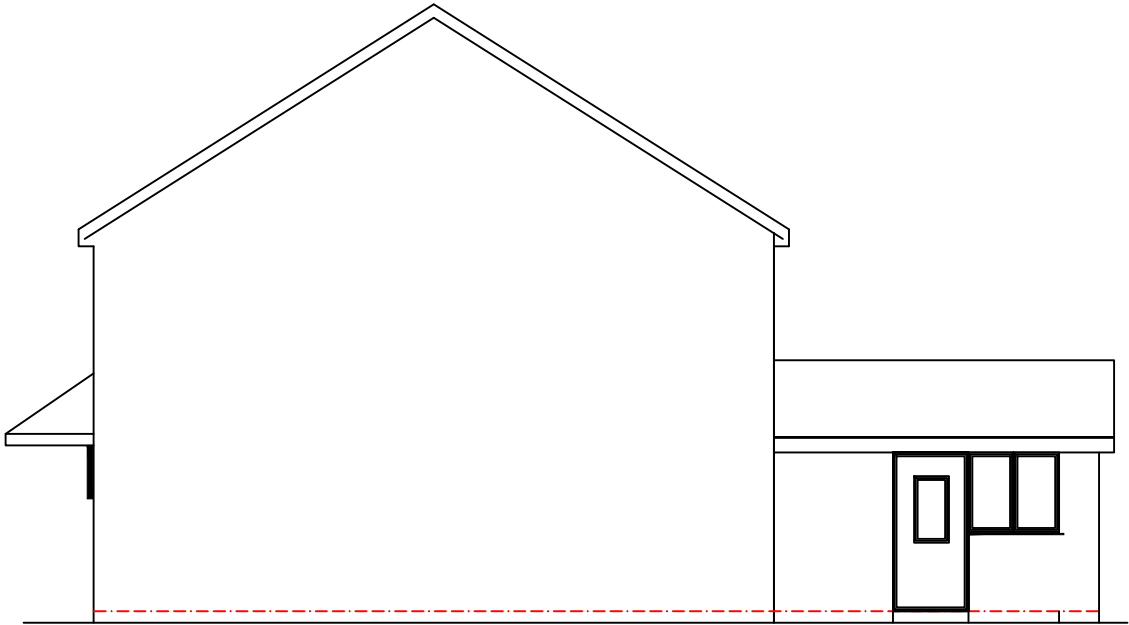
Side Elevation From No 2
