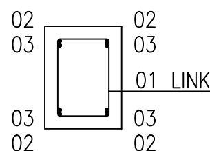
TYPICAL CROSS SECTION
