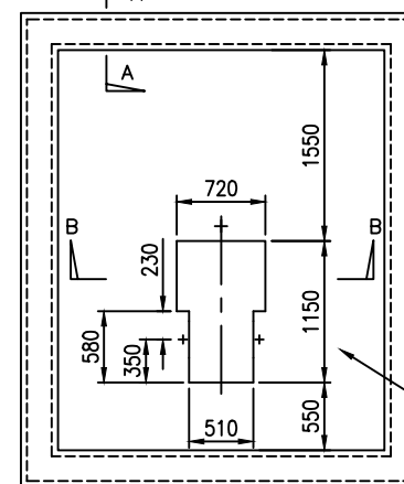
FOUNDATION PLAN
