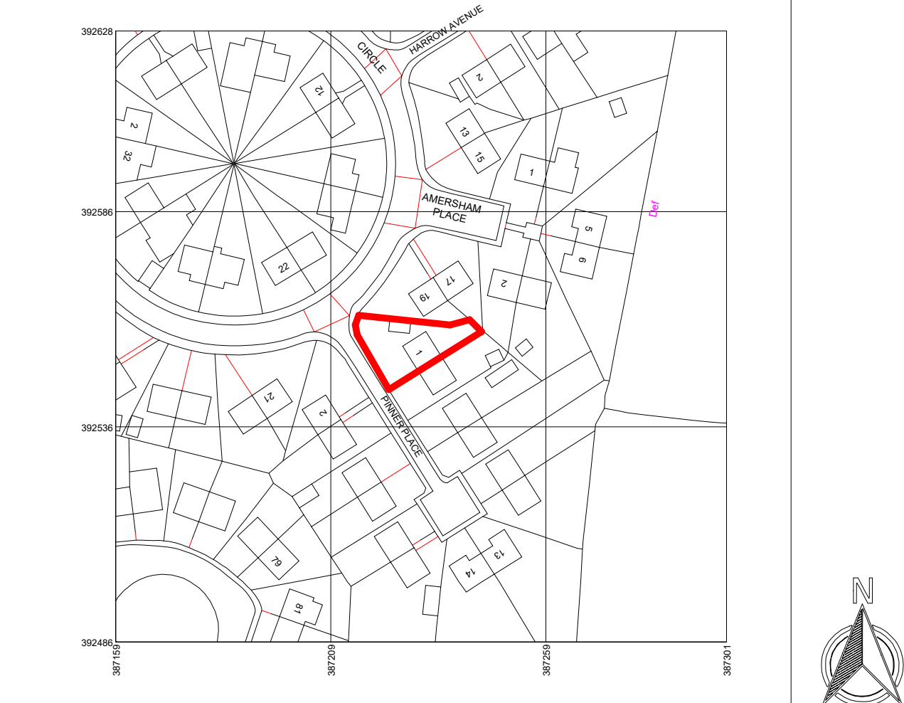
2 LOCATION PLAN 1 : 1250
