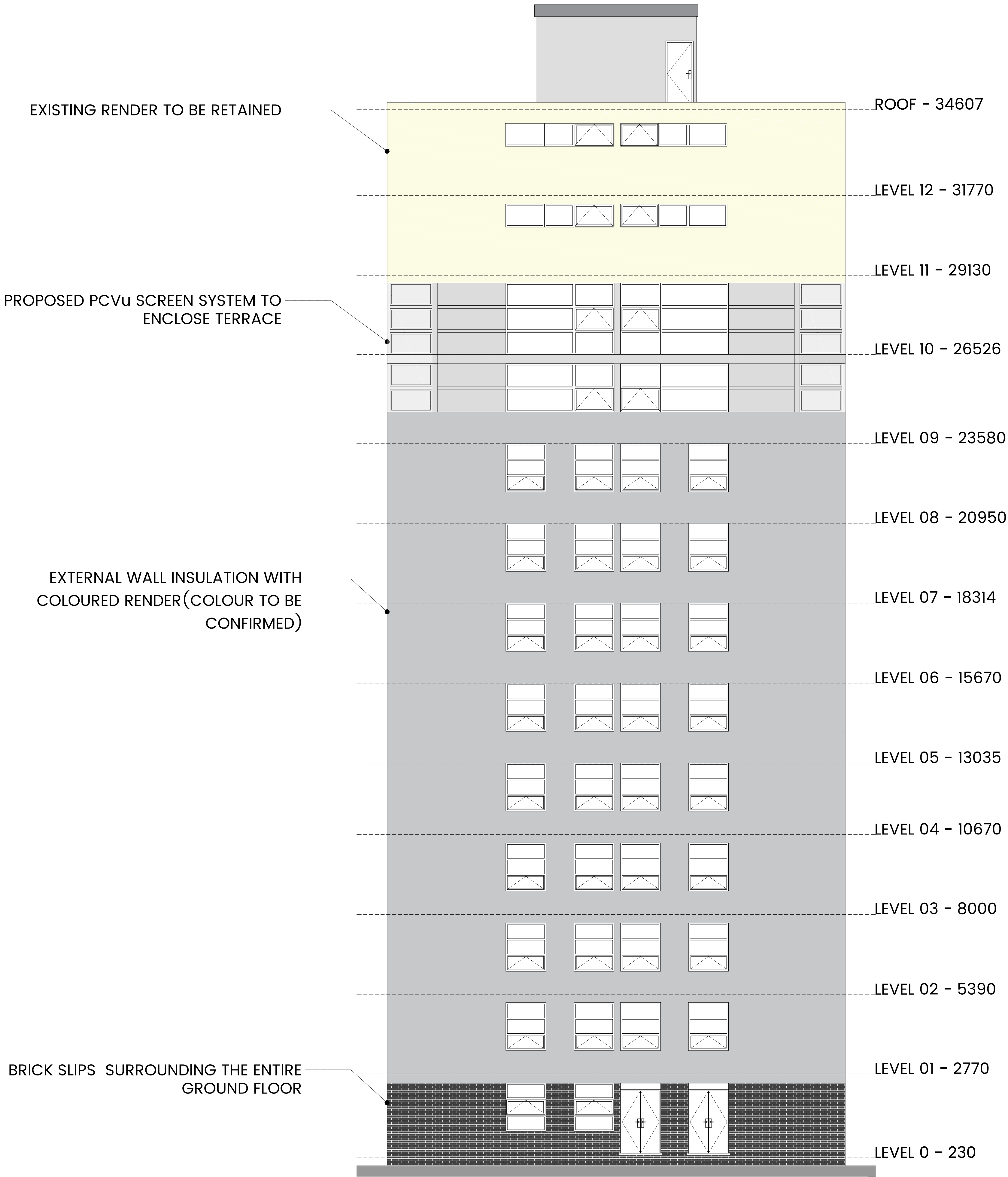
RIGHT HAND SIDE ELEVATION
